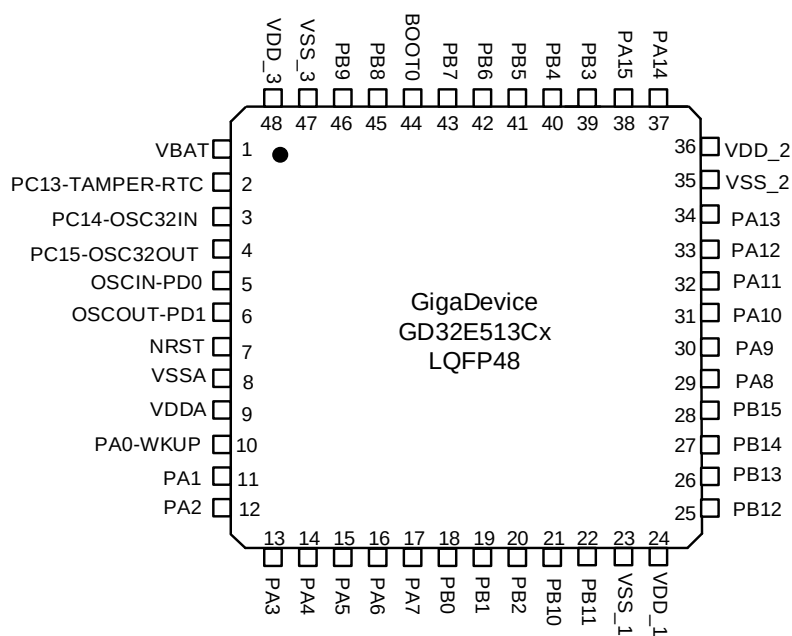
Figure 2-5. GD32E513Cx LQFP48 pinouts
