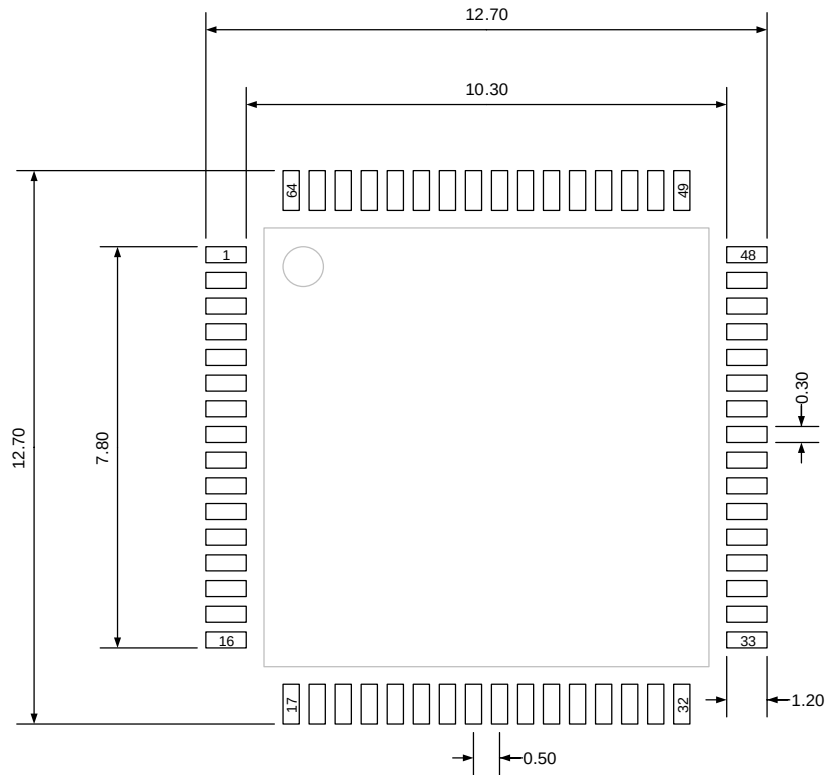
Figure 5-6. LQFP64 recommended footprint
