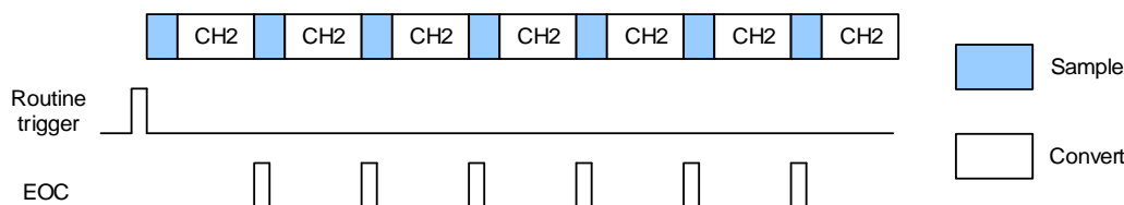
Figure 14-3. Continuous operation mode
