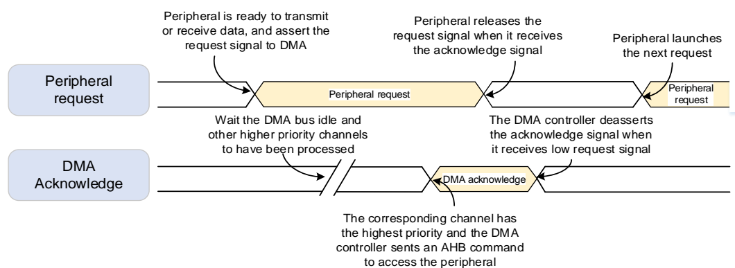
Figure 11-2. Handshake mechanism
