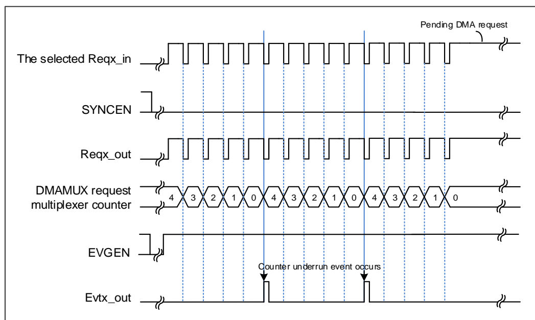
Figure 12-3. Event generation
