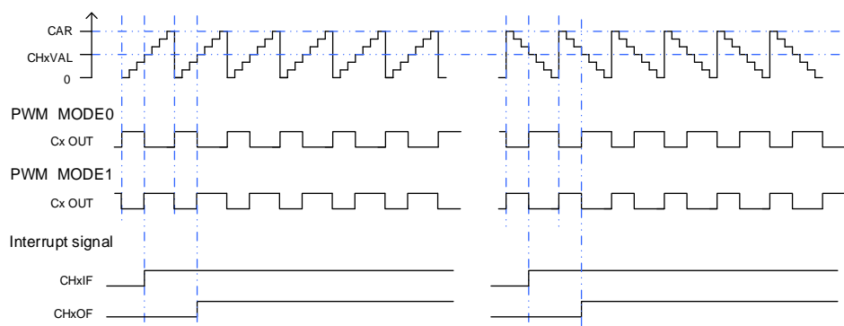
Figure 18-53. EAPWM timechart
