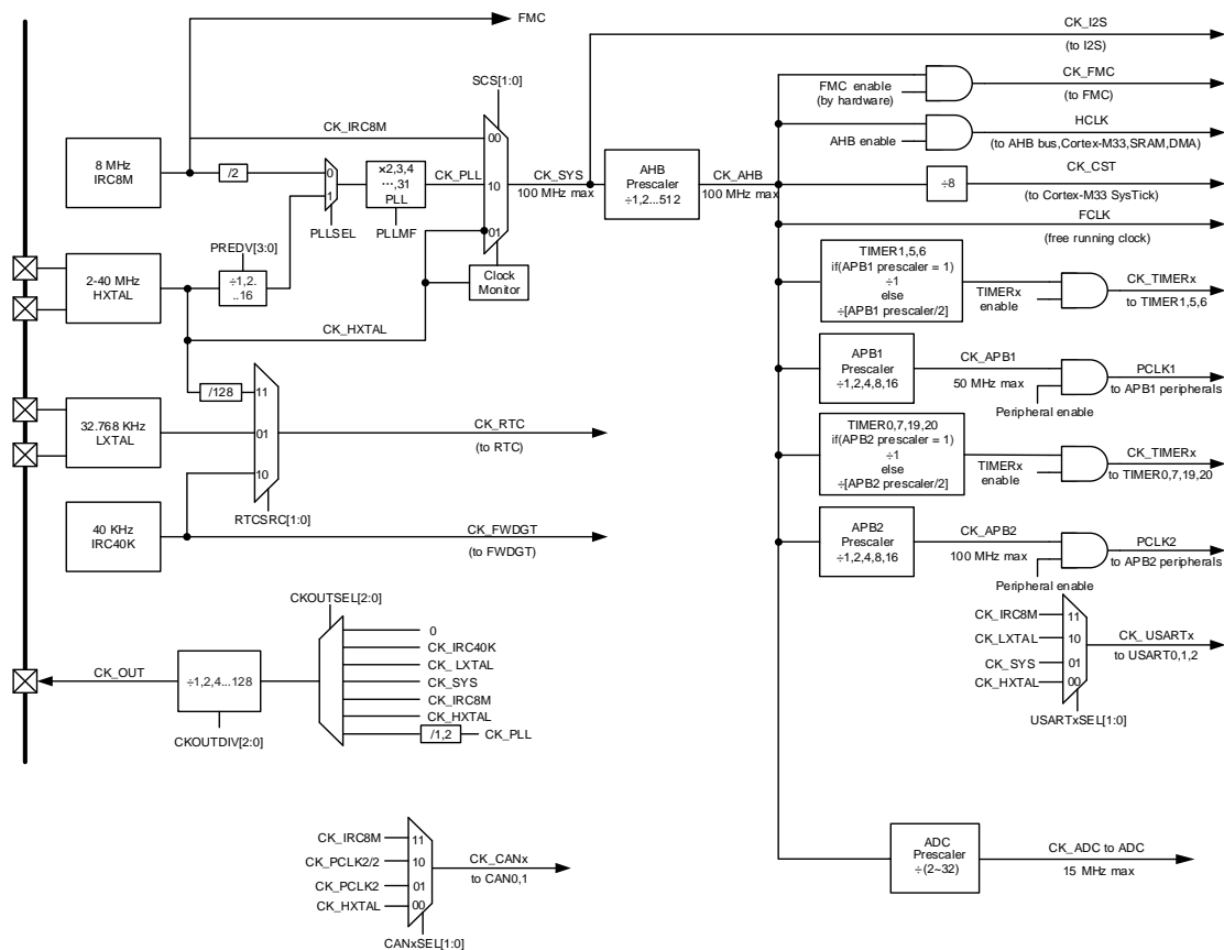
Figure 5-2. Clock tree
