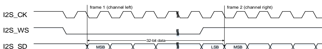
Figure 21-18. I2S Philips standard timing diagram (DTLEN=10, CHLEN=1, CKPL=1)
