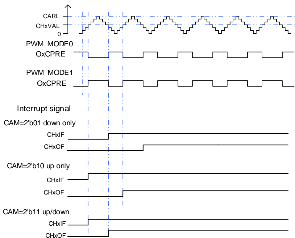
Figure 18-19. CAPWM timechart
