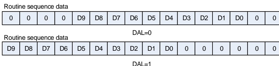
Figure 14-8. Data storage mode of 10-bit resolution
