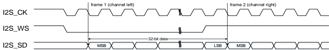
Figure 19-11. I2S Philips standard timing diagram (DTLEN=10, CHLEN=1, CKPL=1)
