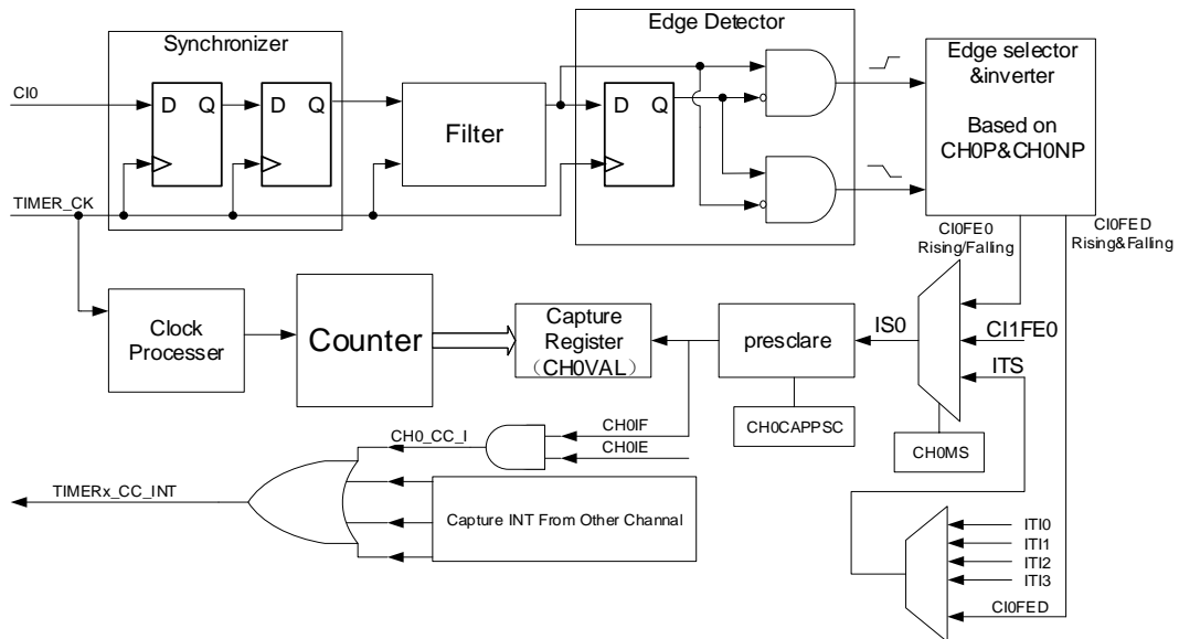
Figure 15-59. Channel input capture principle
