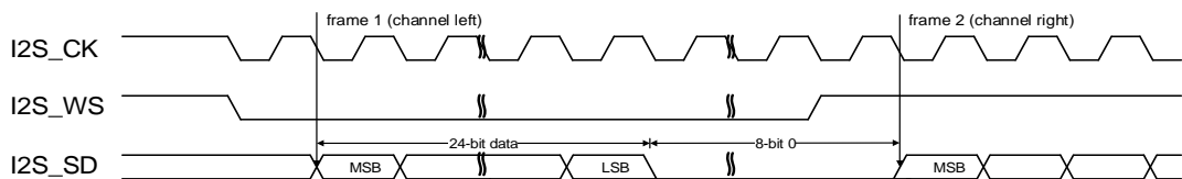
Figure 19-13. I2S Philips standard timing diagram (DTLEN=01, CHLEN=1, CKPL=1)
