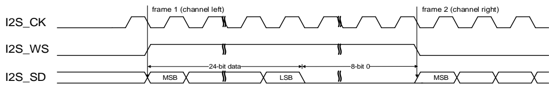
Figure 19-20. MSB justified standard timing diagram (DTLEN=01, CHLEN=1, CKPL=0)
