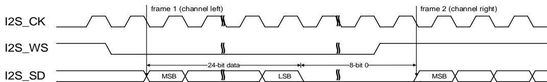
Figure 19-12. I2S Philips standard timing diagram (DTLEN=01, CHLEN=1, CKPL=0)
