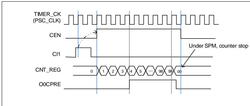
Figure 15-69. Single pulse mode TIMERx\_CHxCV = 4 TIMERx\_CAR=99
