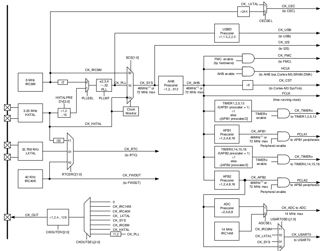
Figure 4-2. Clock tree
