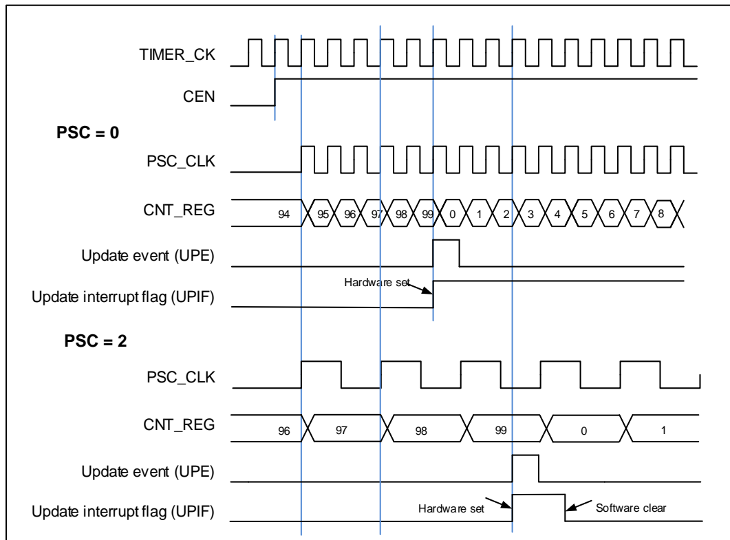
Figure 15-85. Timing chart of up counting mode, PSC=0/2
