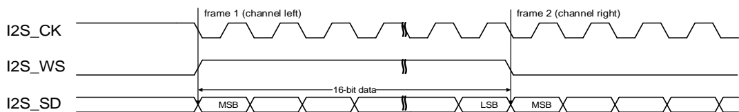
Figure 19-17. MSB justified standard timing diagram (DTLEN=00, CHLEN=0, CKPL=1)
