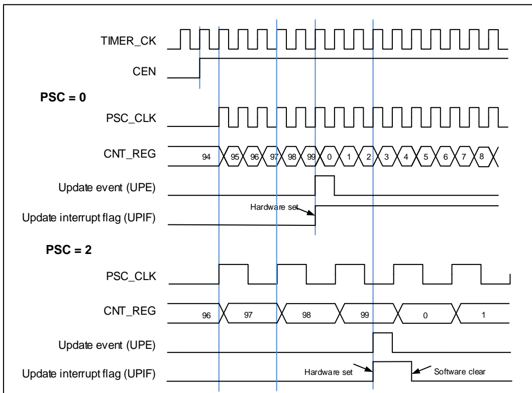
Figure 15-47. Timing chart of up counting mode, PSC=0/2
