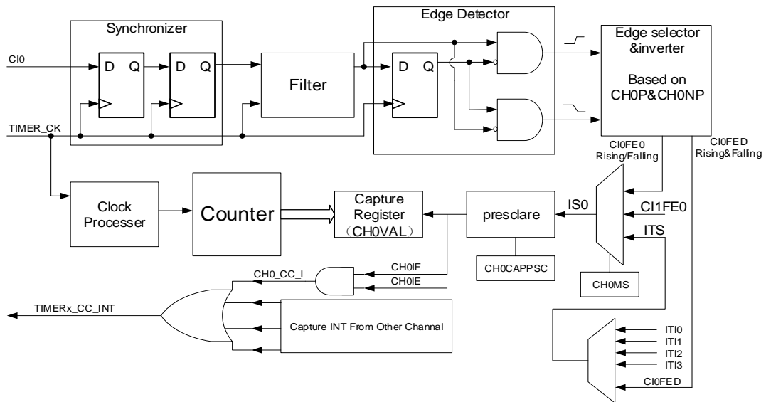
Figure 15-76. Channel input capture principle
