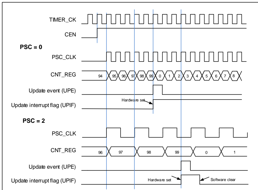
Figure 15-73. Timing chart of up counting mode, PSC=0/2
