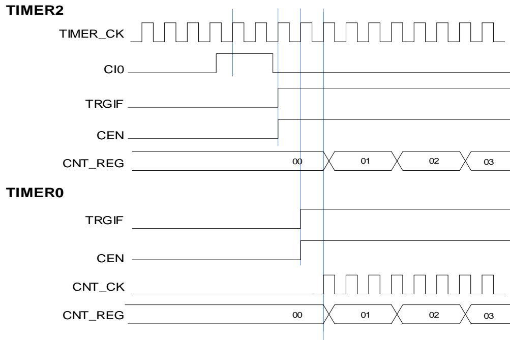
Figure 15-30. Triggering TIMER0 and TIMER2 with TIMER2's CI0 input
