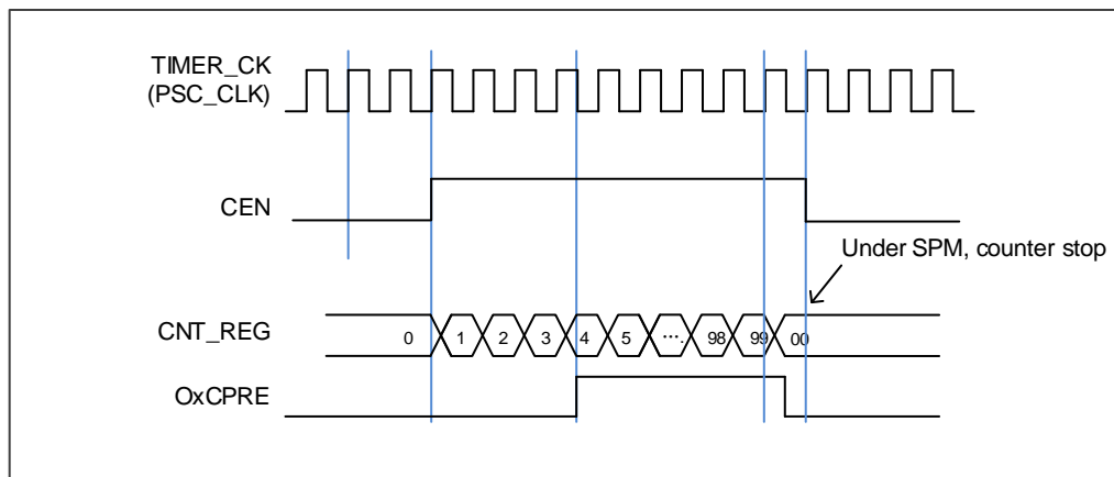
Figure 15-81. Single pulse mode TIMERx_CHxCV = 0x04 TIMERx_CAR=0x60
