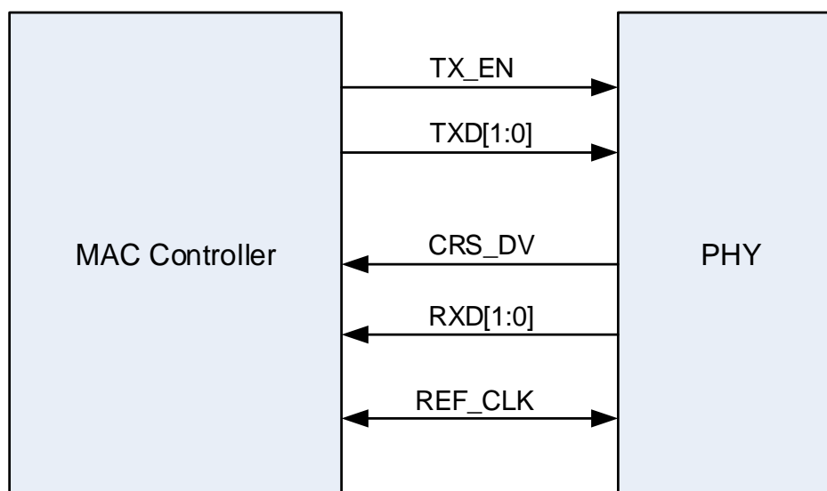
Figure 26-16. Reduced media-independent interface signals
