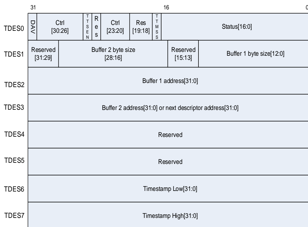
Figure 26-21. Transmit descriptor in enhanced mode
