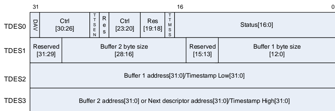
Figure 26-20. Transmit descriptor in normal mode
