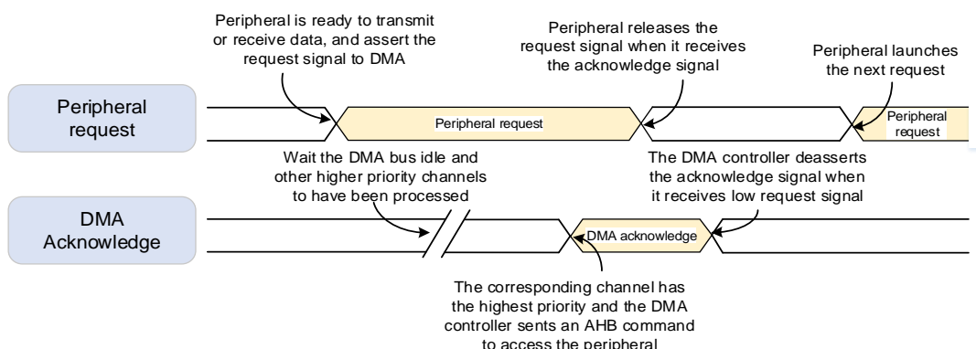
Figure 10-3. Handshake mechanism
