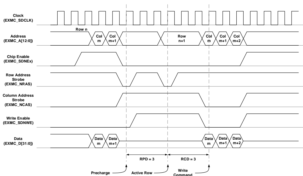
Figure 25-36. Cross boundary write operation
