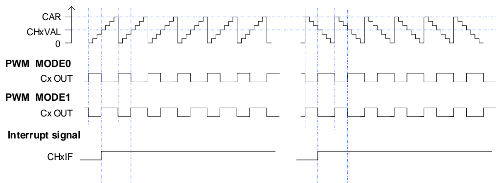
Figure 18-39. CAPWM timechart
