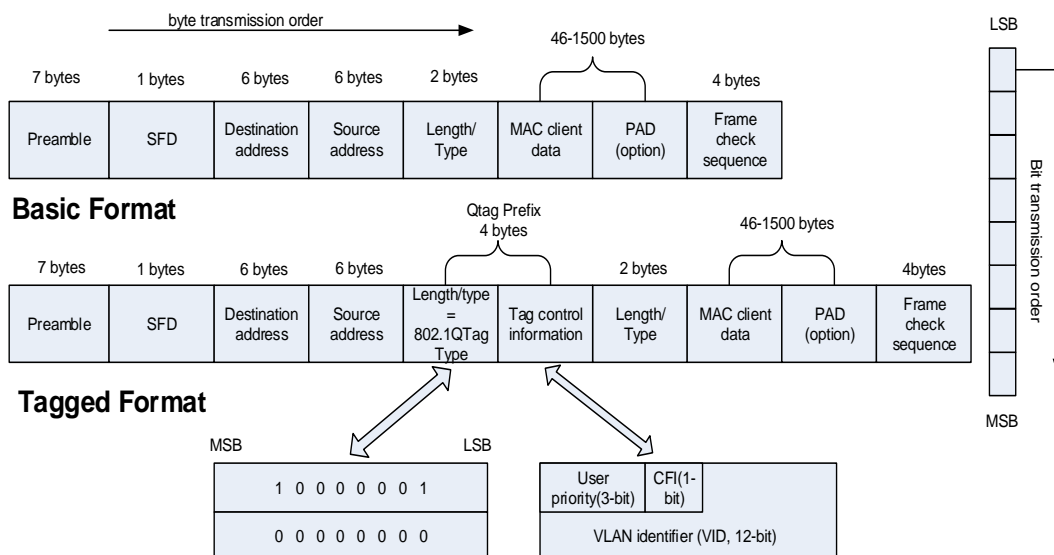
Figure 26-13. MAC / Tagged MAC frame format
