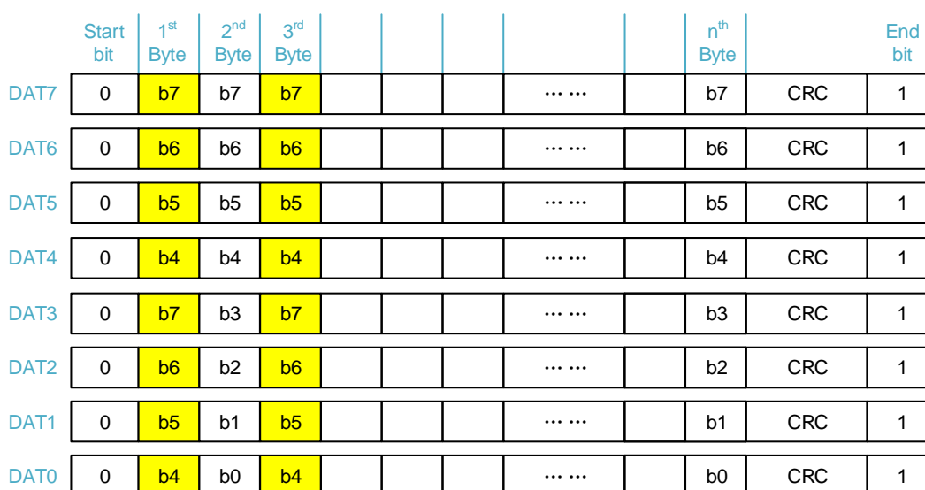
Figure 24-11. 8-bit data bus width
