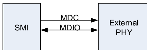
Figure 26-14. Station management interface signals
