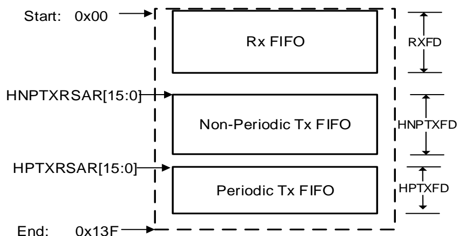
Figure 28-5. HOST mode FIFO space in SRAM
