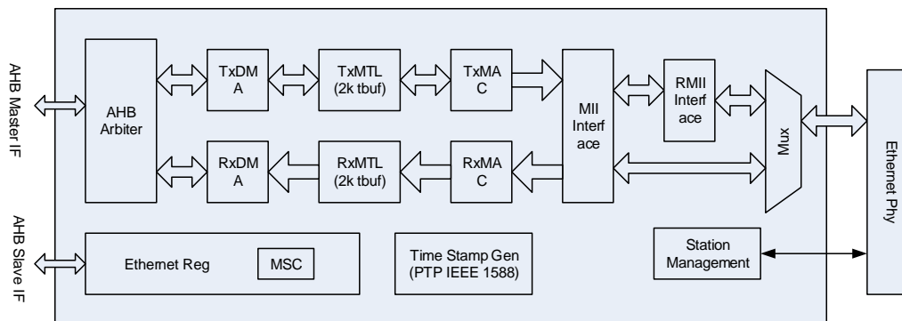
Figure 26-12. ENET module block diagram
