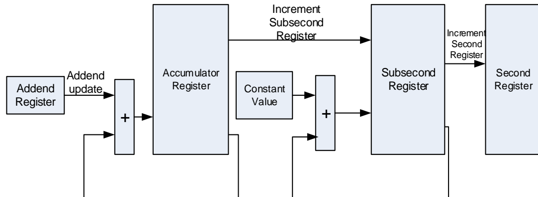
Figure 26-18. System time update using the fine correction method
