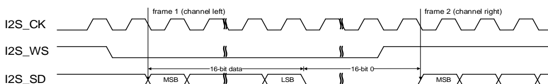
Figure 21-20. I2S Phillips standard timing diagram (DTLEN=00, CHLEN=1, CKPL=0)
