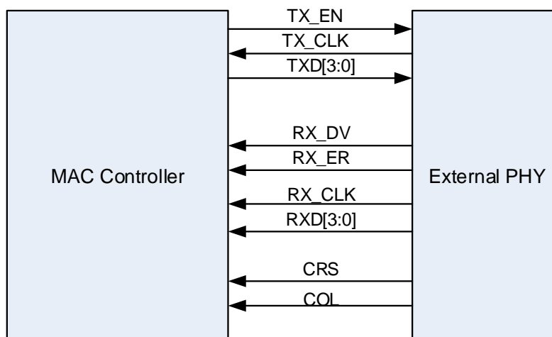
Figure 26-15. Media independent interface signals
