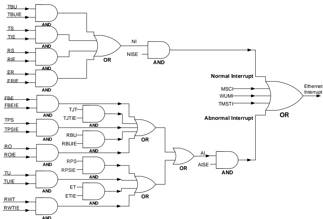
Figure 26-25. Ethernet interrupt scheme
