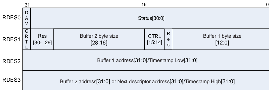
Figure 26-22. Receive descriptor in normal mode
