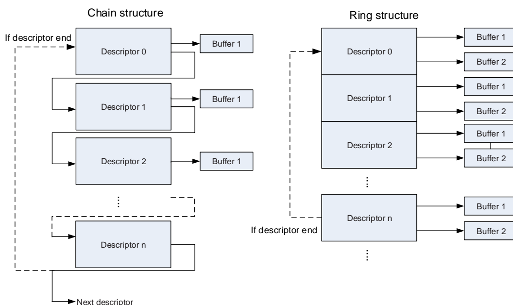
Figure 26-19. Descriptor ring and chain structure
