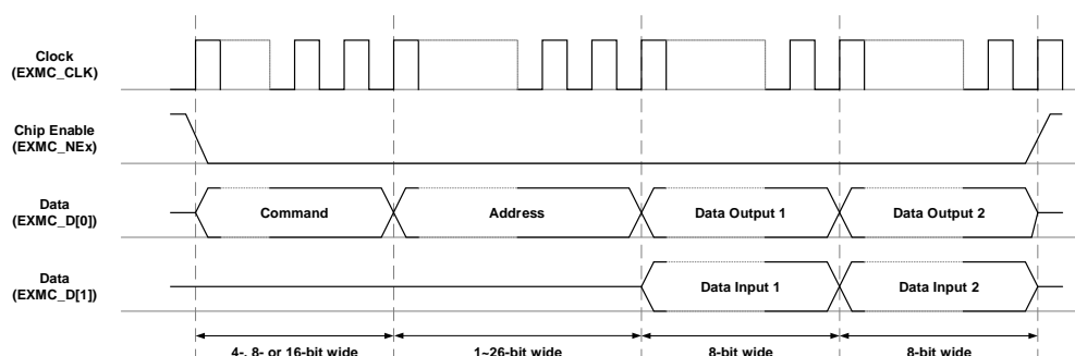
Figure 25-24. SPI-PSRAM access
