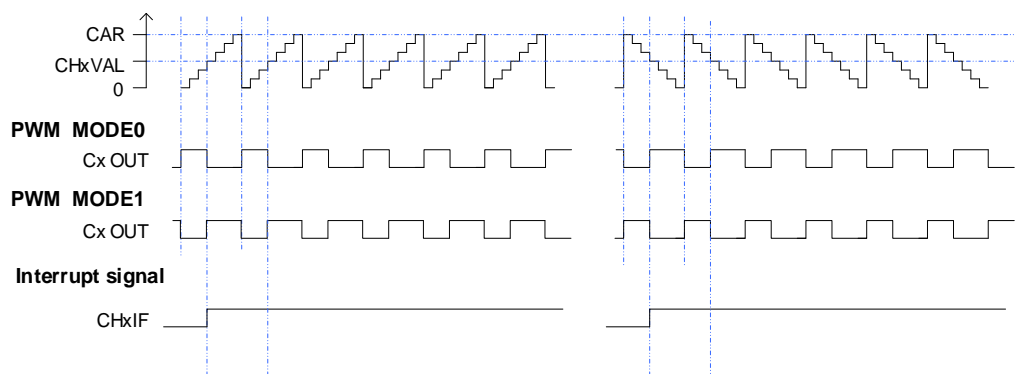
Figure 18-51. CAPWM timechart
