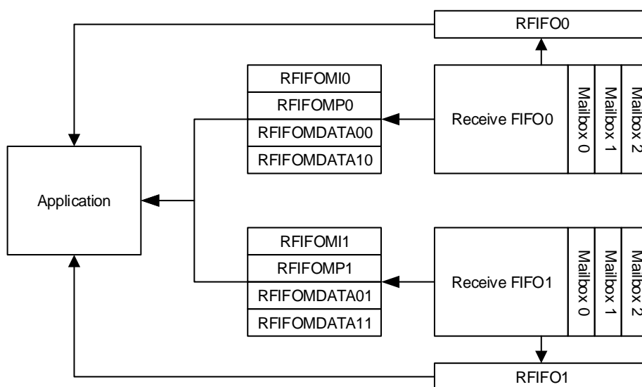
Figure 26-4. Reception register
