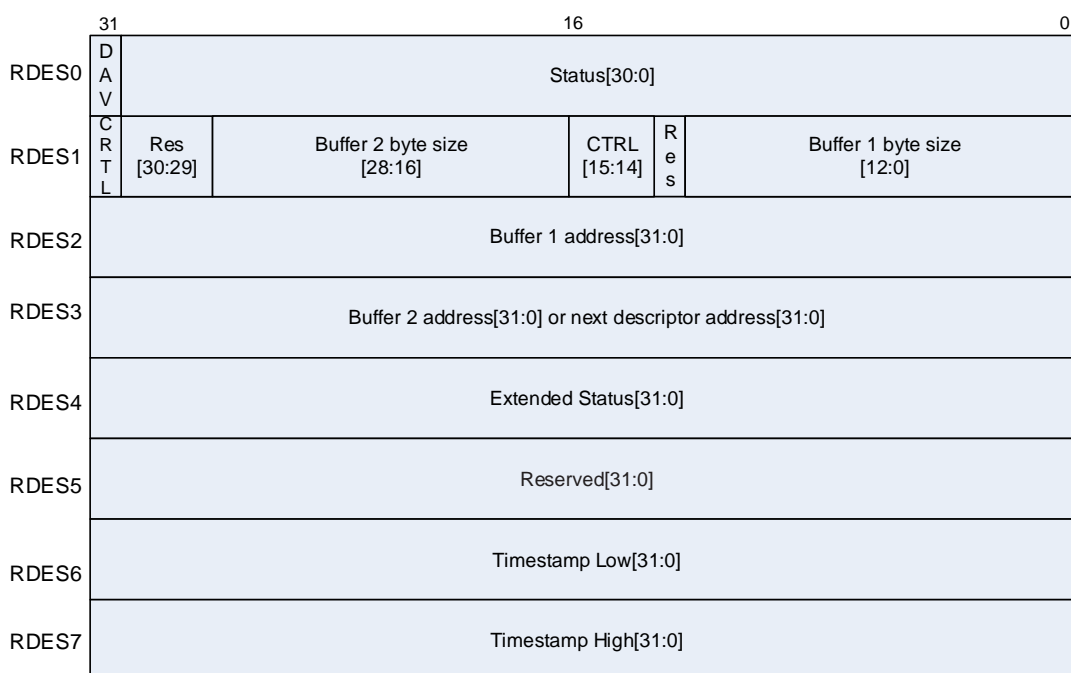
Figure 26-23. Receive descriptor in enhanced mode
