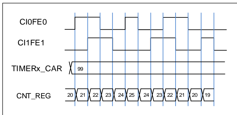
Figure 18-18. Counter behavior with CI0FE0 polarity non-inverted in mode 2
