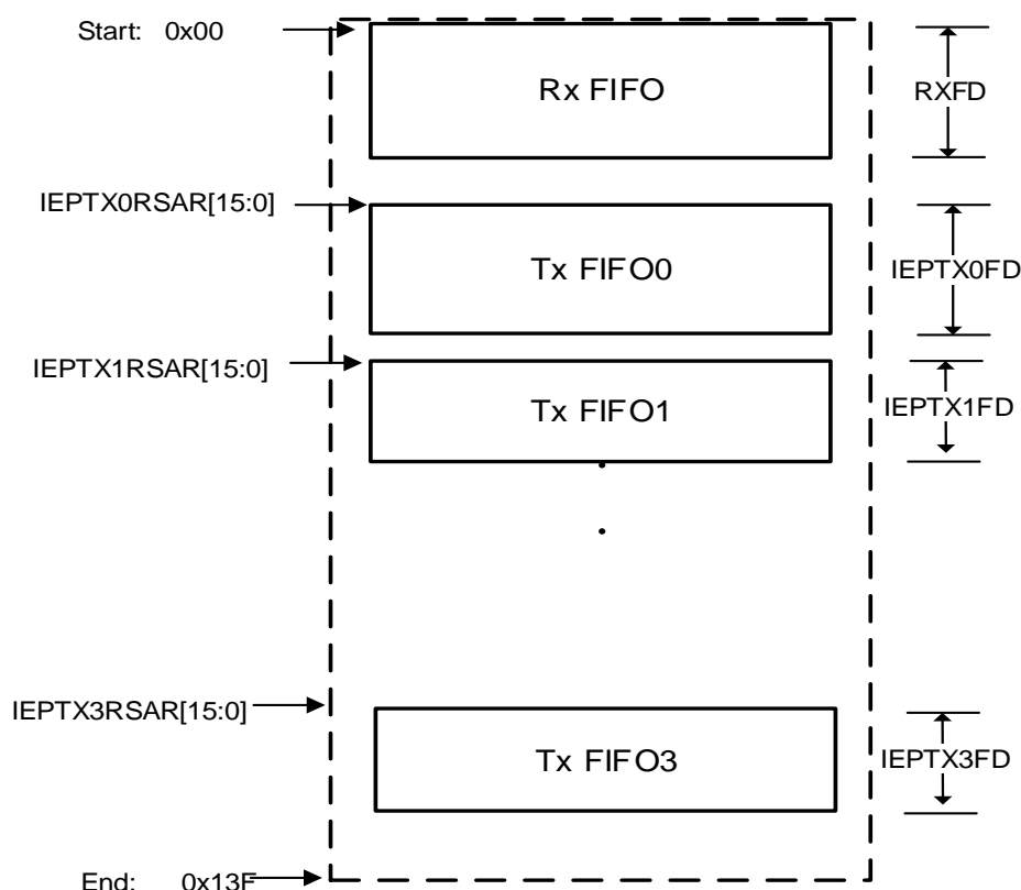
Figure 28-7. Device mode FIFO space in SRAM
