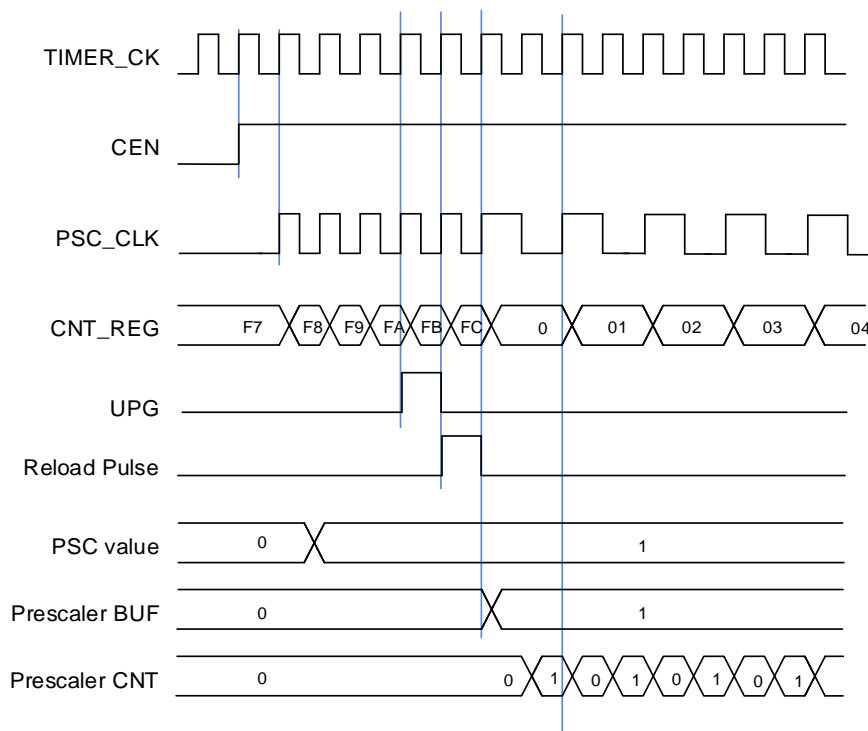
Figure 23-96. Counter timing diagram with prescaler division change from 1 to 2
