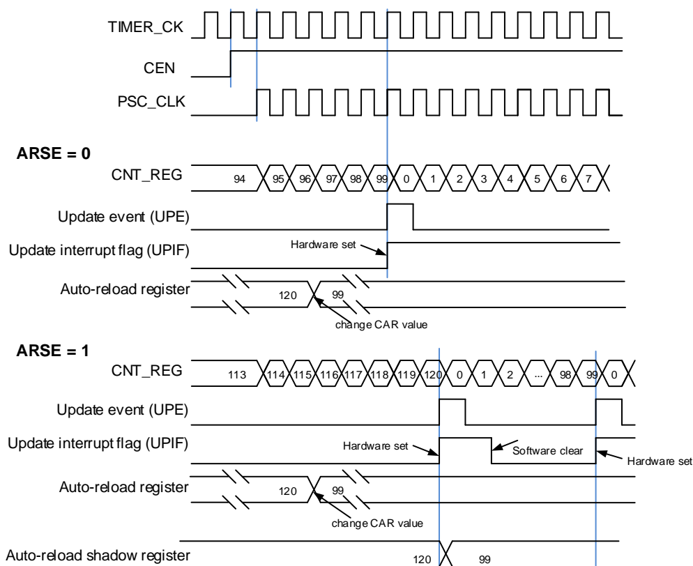
Figure 23-147. Timing chart of up counting mode, change TIMERx_CAR ongoing
