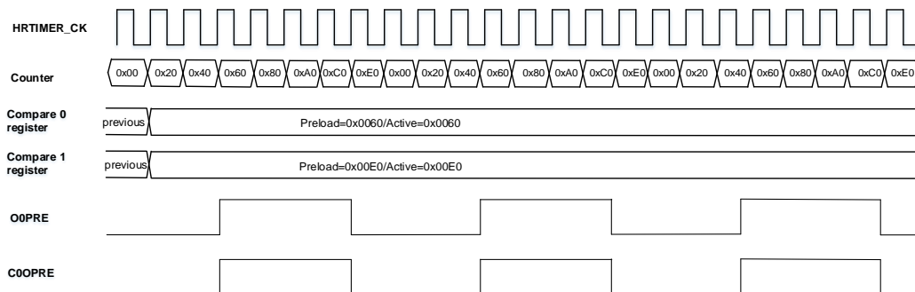
Figure 25-29. C0OPRE wave in regular mode
