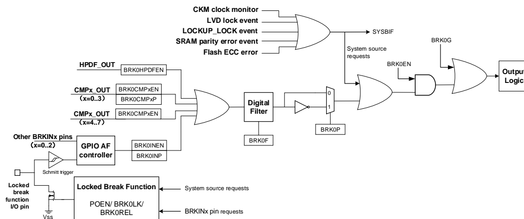
Figure 23-141. BRKIN0 pin logic with BREAK0 function
