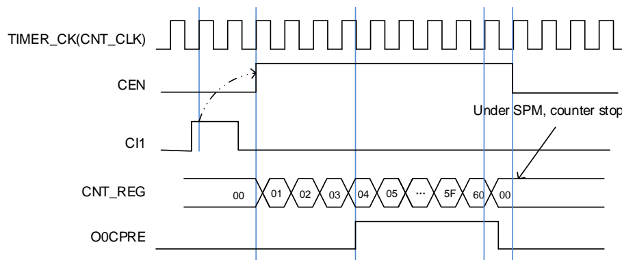
Figure 23-92. Single pulse mode TIMERx\_CHxCV = 0x04 , TIMERx\_CAR=0x60
