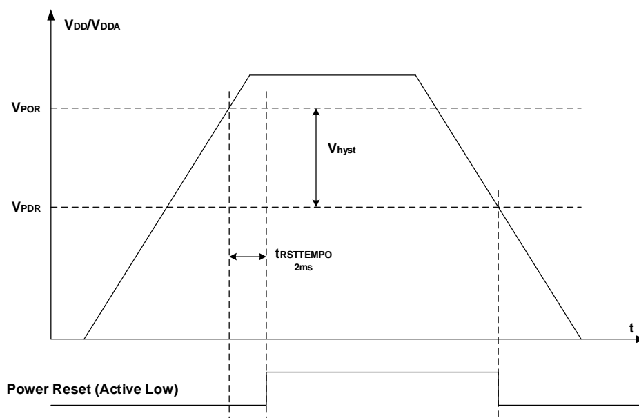
Figure 3-4. Waveform of the POR/PDR
