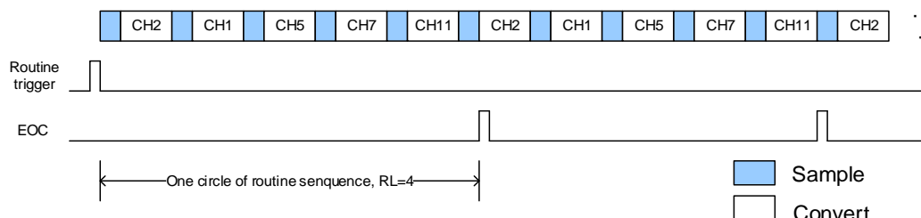
Figure 17-5. Scan operation mode, continuous enable
