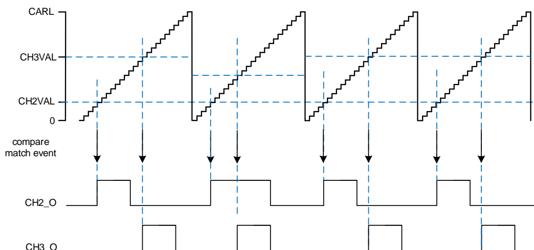
Figure 23-56. CH2_O and CH3_O output the pulse at the same time
