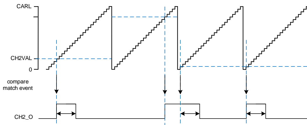
Figure 23-55. Programmable pulse output circuitry waveform
