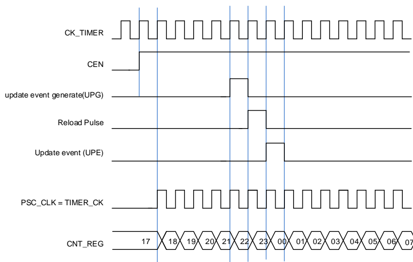
Figure 23-66. Normal mode, internal clock divided by 1
