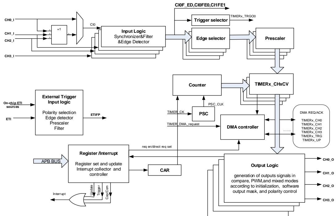
Figure 23-65. General Level 0 timer block diagram
