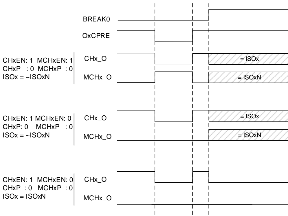
Figure 23-140. Output behavior of the channel in response to BREAK0 (the break input high active and IOS=1)
