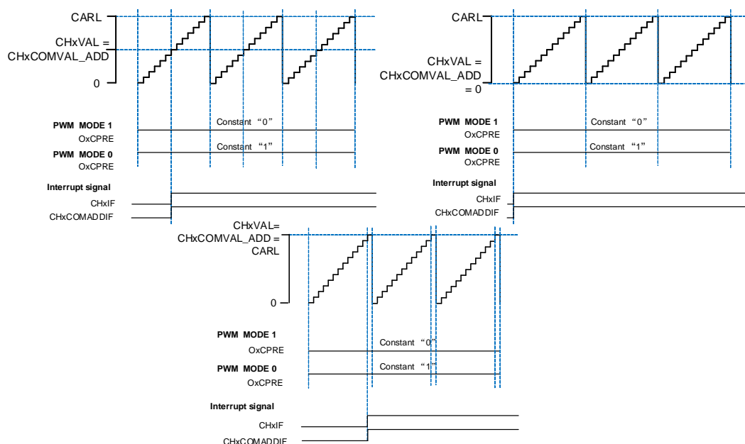
Figure 23-110. Channel x output PWM with (CHxVAL = CHxCOMVAL_ADD)
