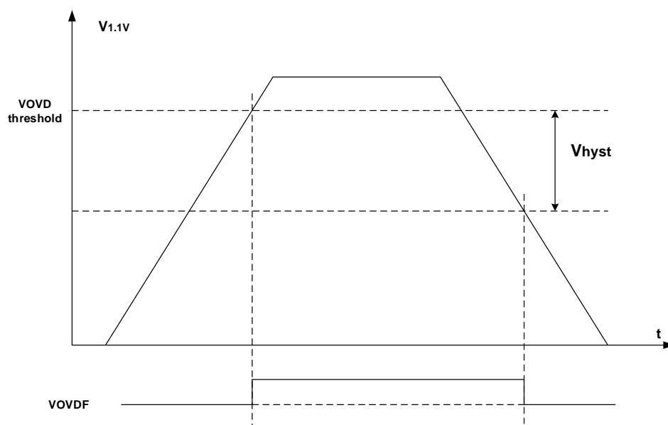
Figure 3-8. waveform of VOVD
