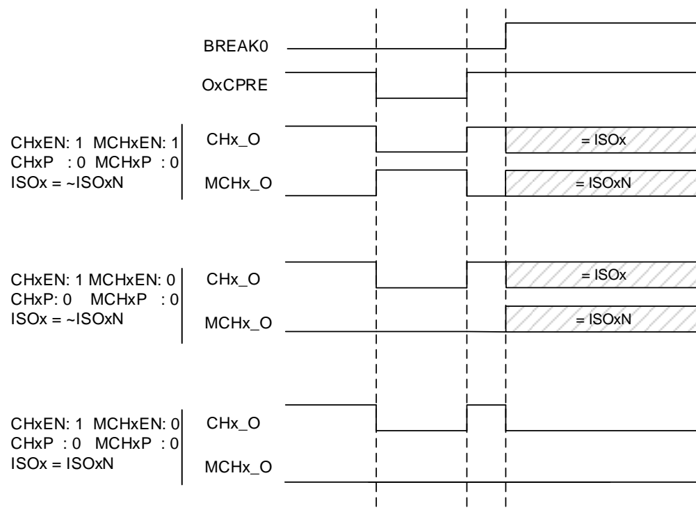
Figure 23-34. Output behavior of the channel in response to BREAK0 (the break input high active and IOS=1)
