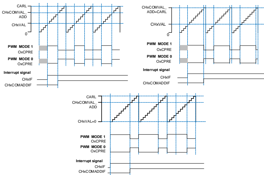
Figure 23-81. Channel x output PWM with (CHxVAL < CHxCOMVAL_ADD)
