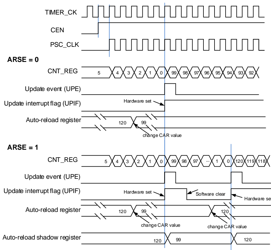
Figure 23-71. Timing chart of down counting mode, change TIMERx_CAR ongoing
