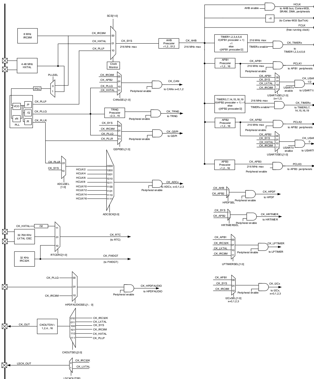
Figure 4-2. Clock tree
