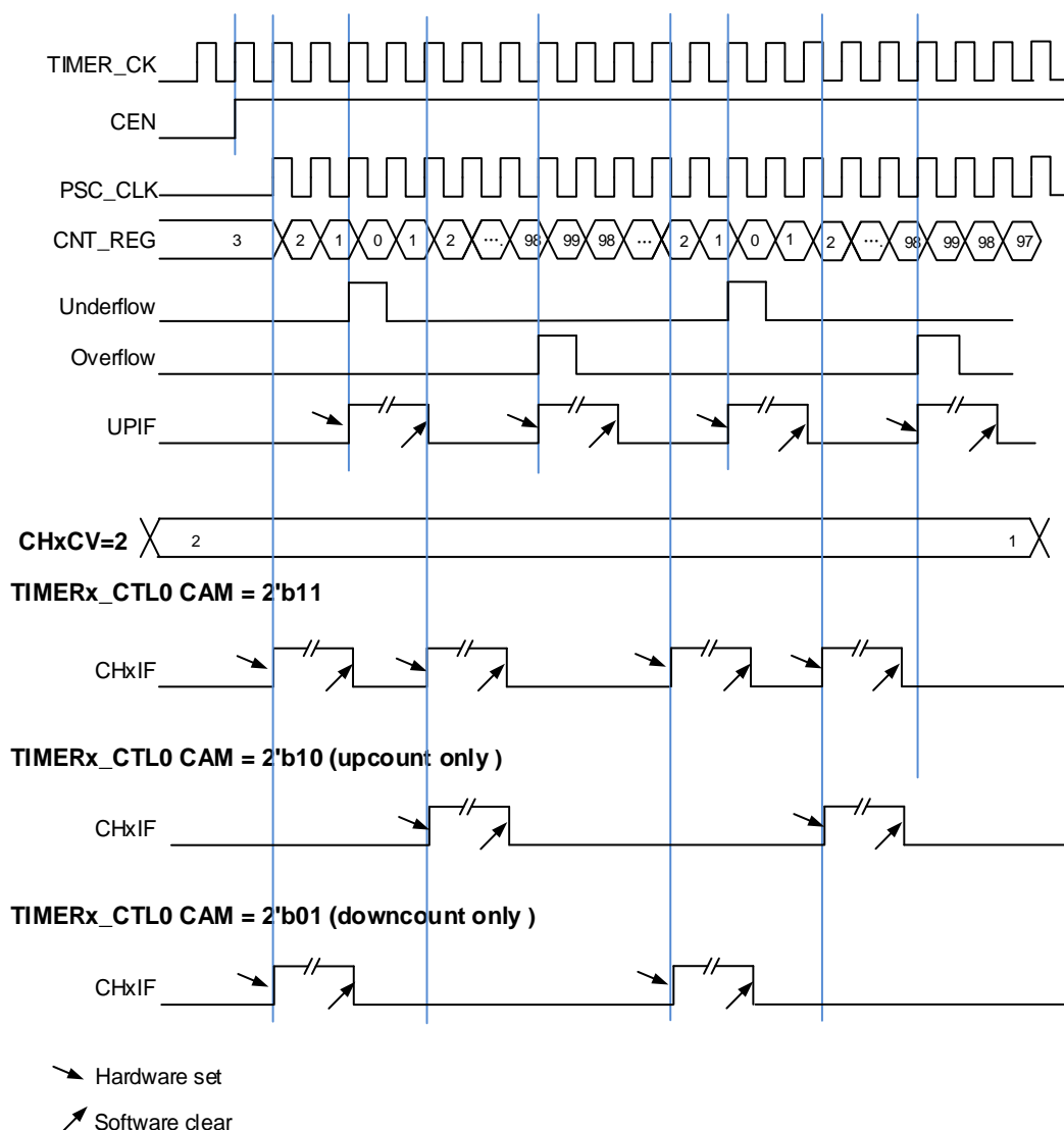
Figure 23-72. Timing chart of center-aligned counting mode
