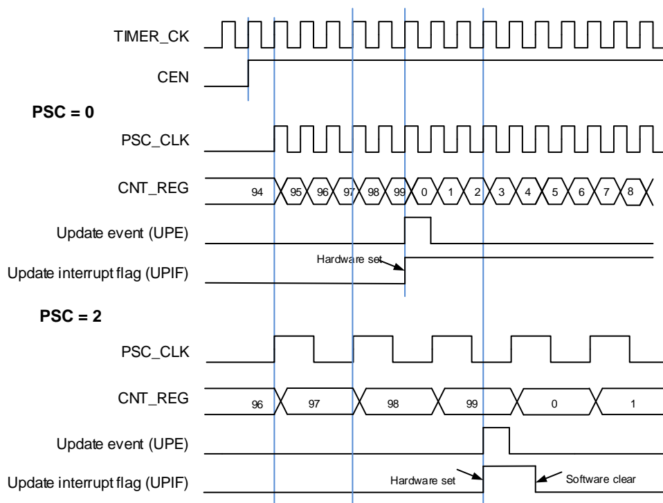
Figure 23-146. Timing chart of up counting mode, PSC=0/1
