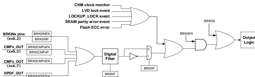
Figure 23-117. BREAK0 function logic diagram
