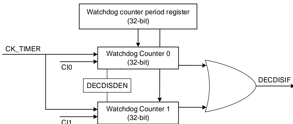
Figure 23-39. Quadrature decoder signal disconnection detection block diagram
