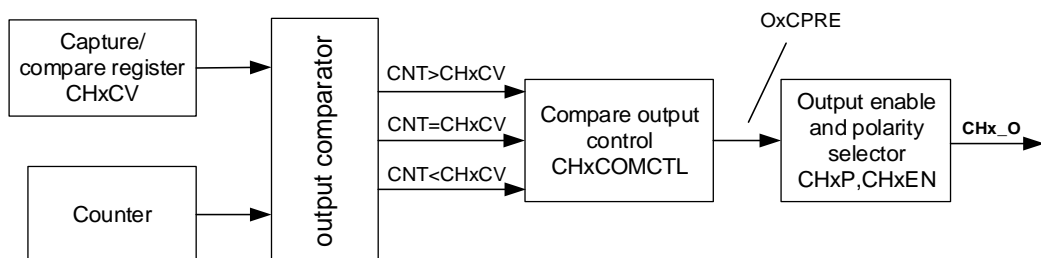
Figure 23-104. Output compare logic (x=1)
