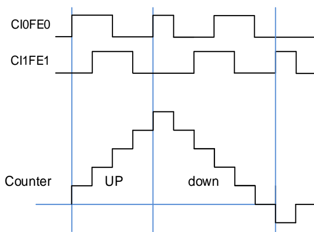
Figure 23-37. Example of counter operation in decoder interface mode
