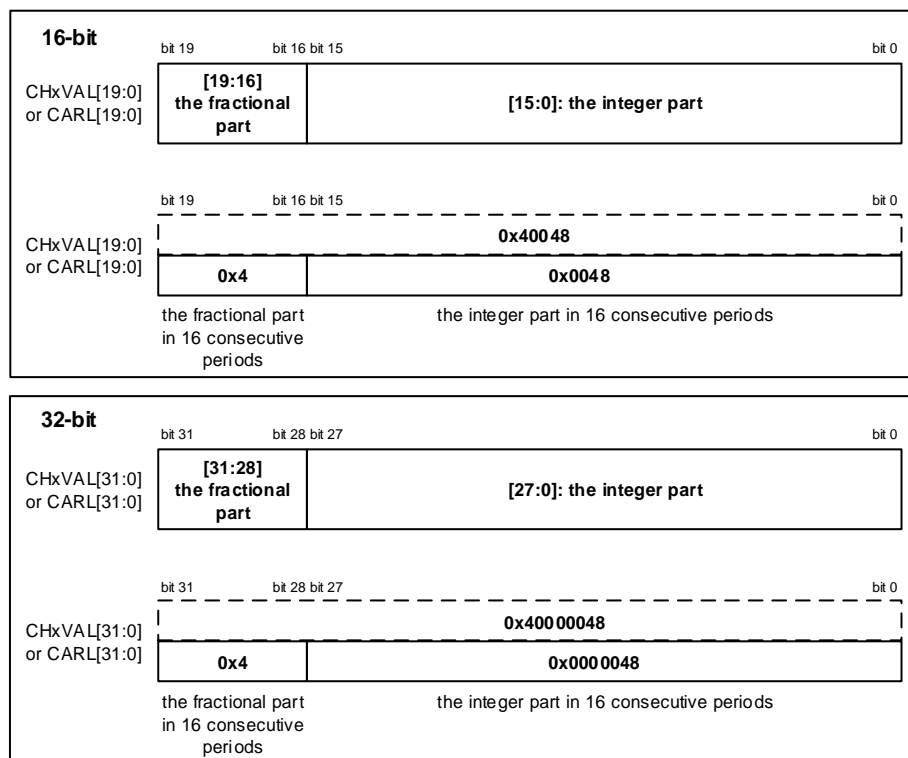
Figure 23-78. Adjustment mode: Data format and the register bit-field
