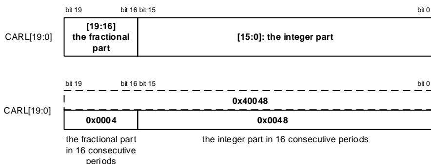
Figure 23-148. Adjustment mode: Data format and the register bit-field
