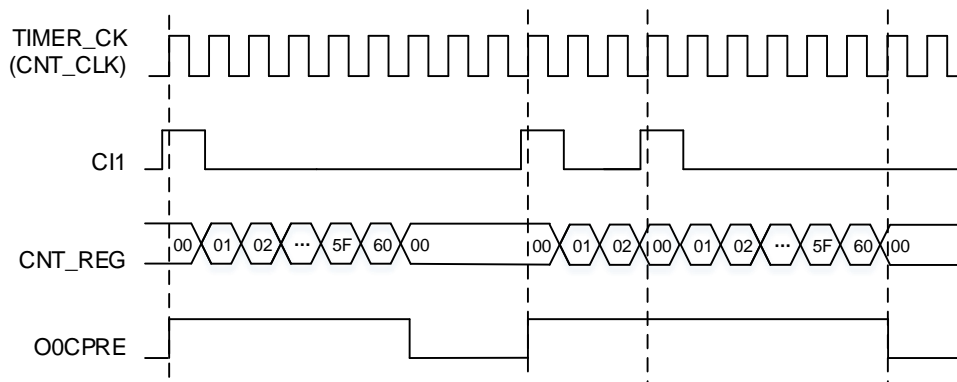
Figure 23-53. delayable single pulse mode with TIMERx_CHxCV=0x00, TIMERx_CAR=0x60
