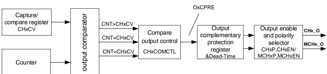
Figure 23-103. Output compare logic (when MCHxMSEL = 2'b11, x=0)
