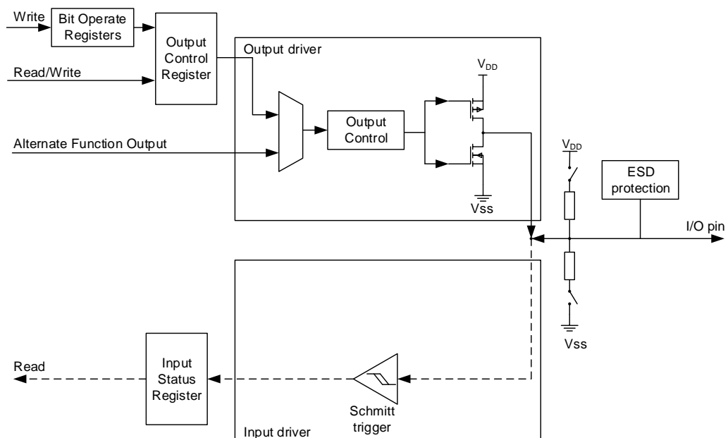
Figure 7-3. Output configuration
