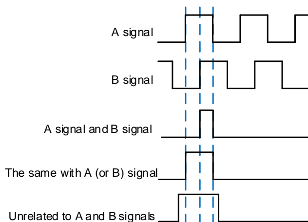
Figure 23-42. Three types of index signals
