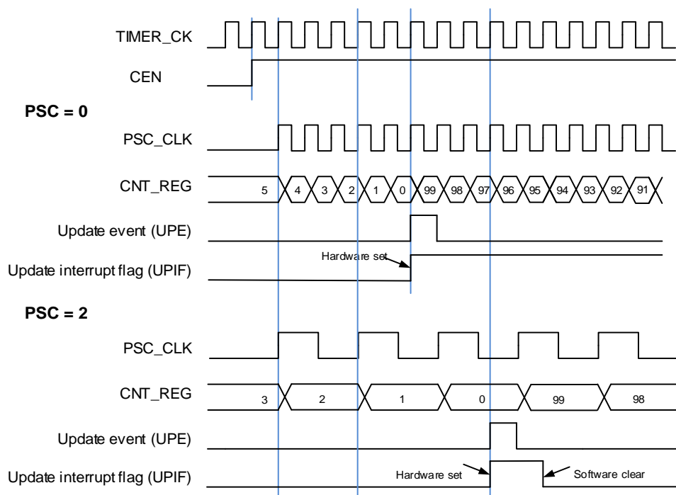
Figure 23-70. Timing chart of down counting mode, PSC=0/2
