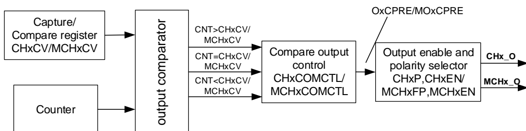
Figure 23-15. Output compare logic (when MCHxMSEL = 2'b11, x=0,1,2,3)
