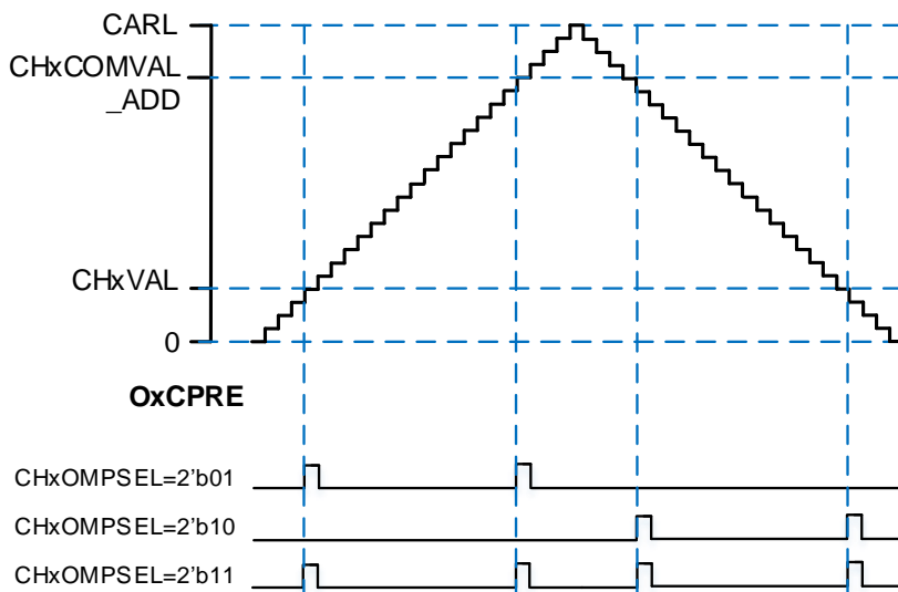
Figure 23-88. CHx_O output with a pulse in center-aligned mode (CHxOMPSEL#2'b00)
