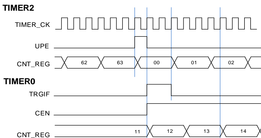
Figure 23-58. Trigger mode of TIMER0 controlled by update signal of TIMER2
