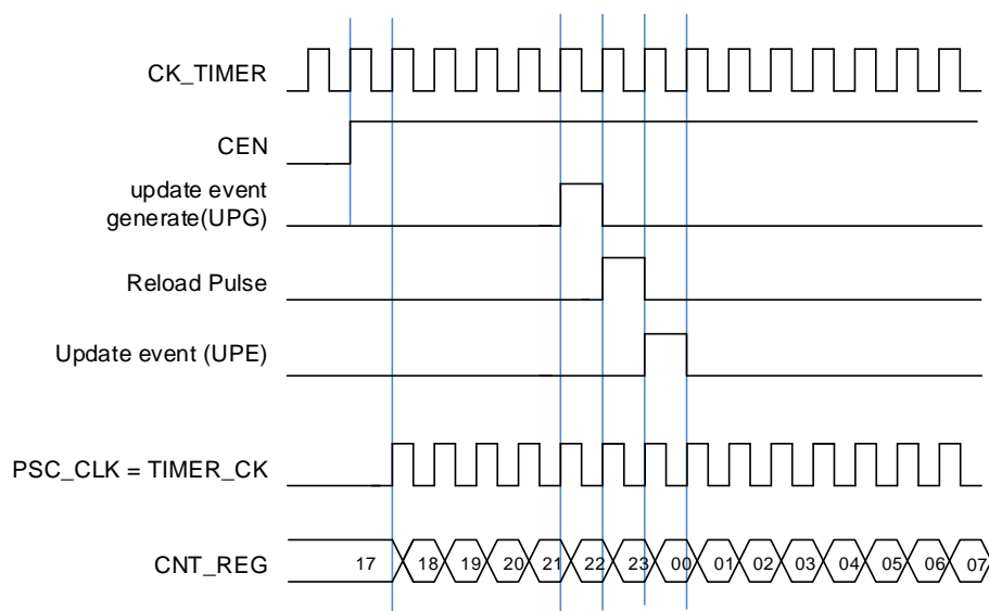
Figure 23-95. Normal mode, internal clock divided by 1
