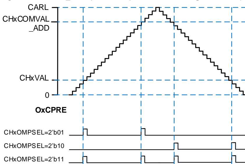
Figure 23-29. CHx_O output with a pulse in center-aligned mode (CHxOMPSEL#2'b00)
