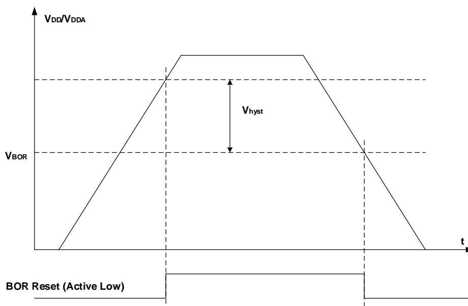
Figure 3-5. Waveform of the BOR
