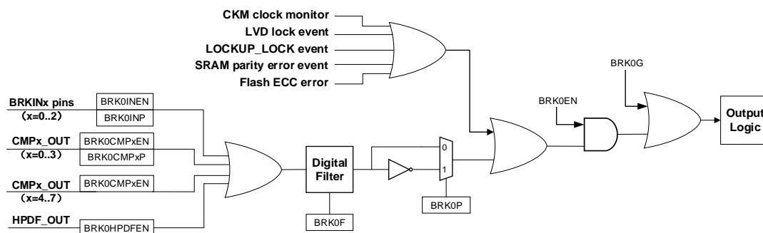
Figure 23-139. BREAK0 function logic diagram
