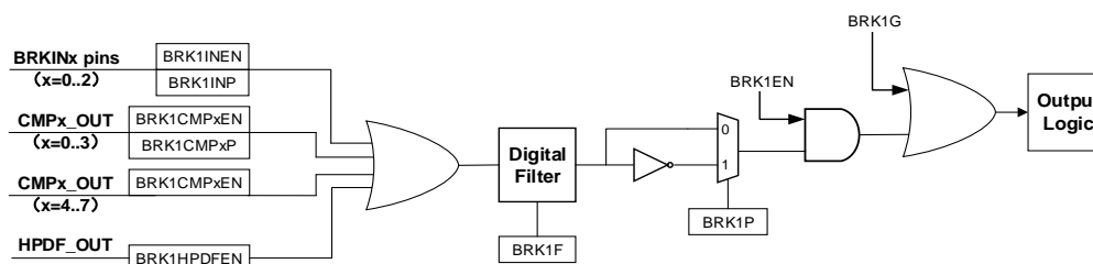
Figure 23-33. BREAK1 function logic diagram
