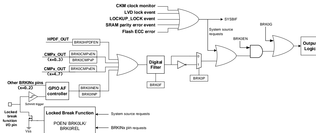
Figure 23-119. BRKIN0 pin logic with BREAK0 function
