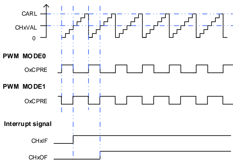
Figure 23-106. PWM mode timechart
