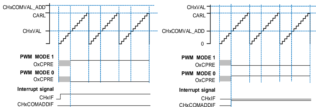
Figure 23-84. Channel x output PWM with CHxVAL or CHxCOMVAL_ADD exceeds CARL
