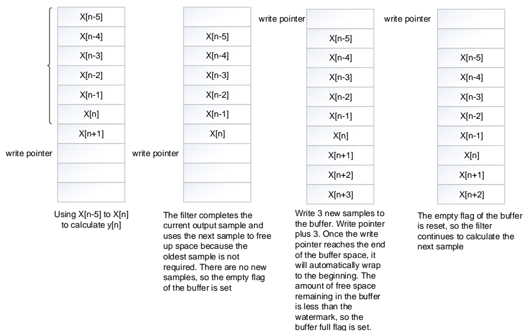
Figure 35-4 Circular input buffer operation
