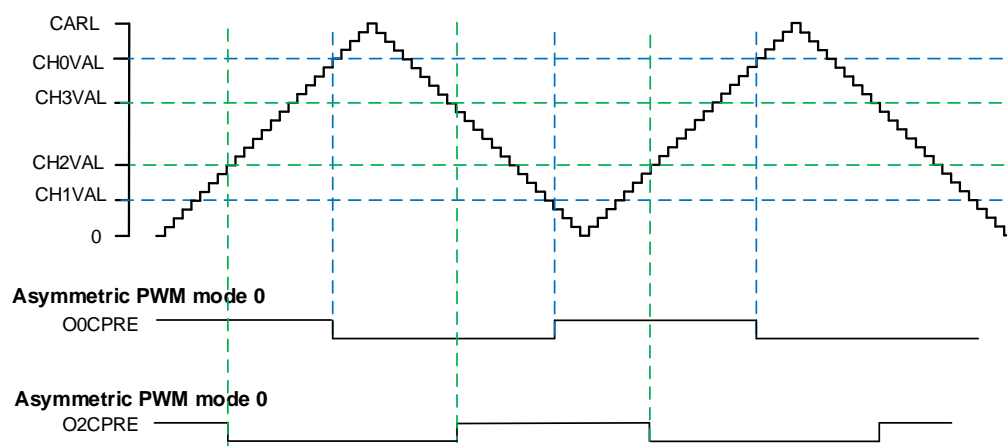
Figure 23-21. CH0 and CH2 with asymmetric PWM mode
