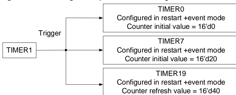
Figure 23-62. Configurable phase method diagram
