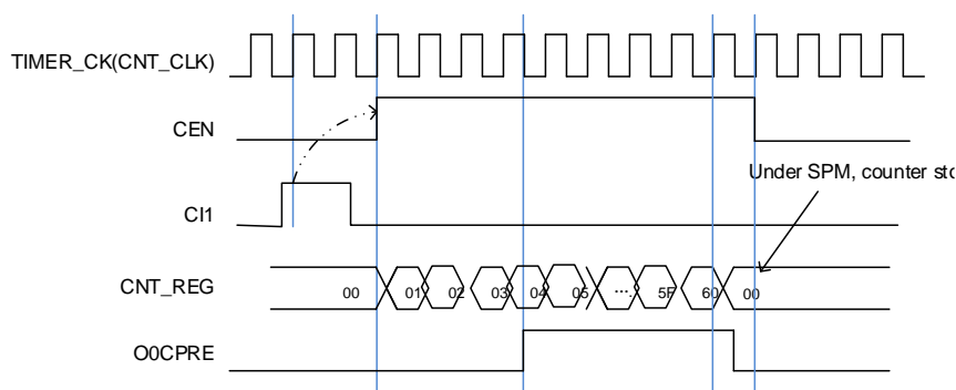
Figure 23-142. Single pulse mode TIMERx_CHxCV = 0x04 TIMERx_CAR=0x60
