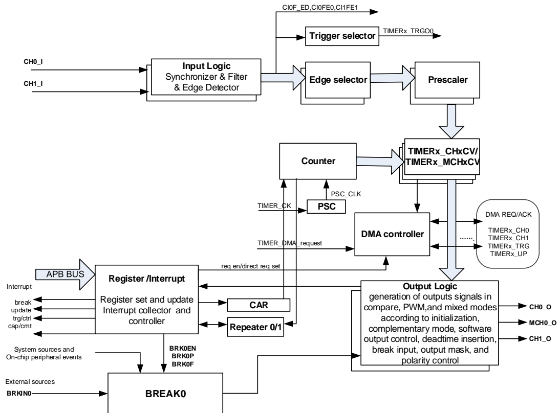
Figure 23-94. General level3 timer block diagram
