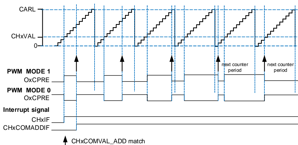
Figure 23-26. Channel x output PWM duty cycle changing with CHxCOMVAL_ADD
