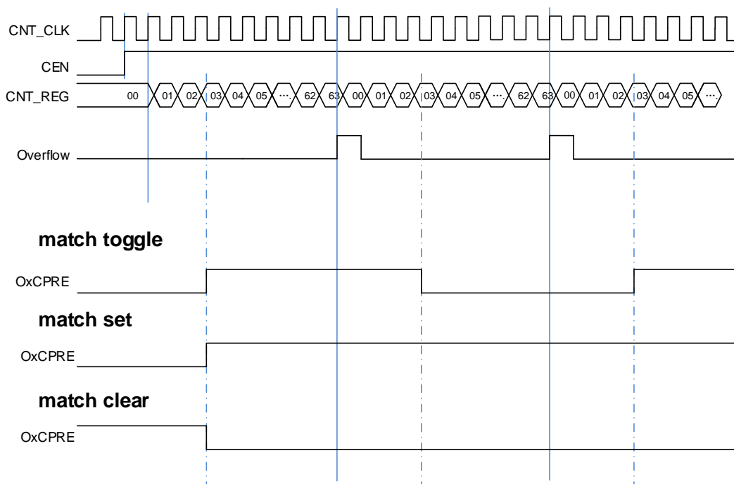
Figure 23-135. Output-compare in three modes
