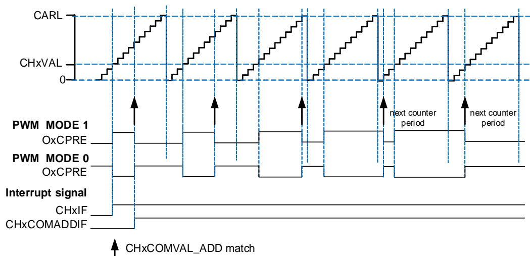
Figure 23-113. Channel x output PWM duty cycle changing with CHxCOMVAL_ADD
