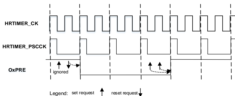
Figure 25-28. OXPRE wave with CNTCKDIV[2:0] = 3'b110
