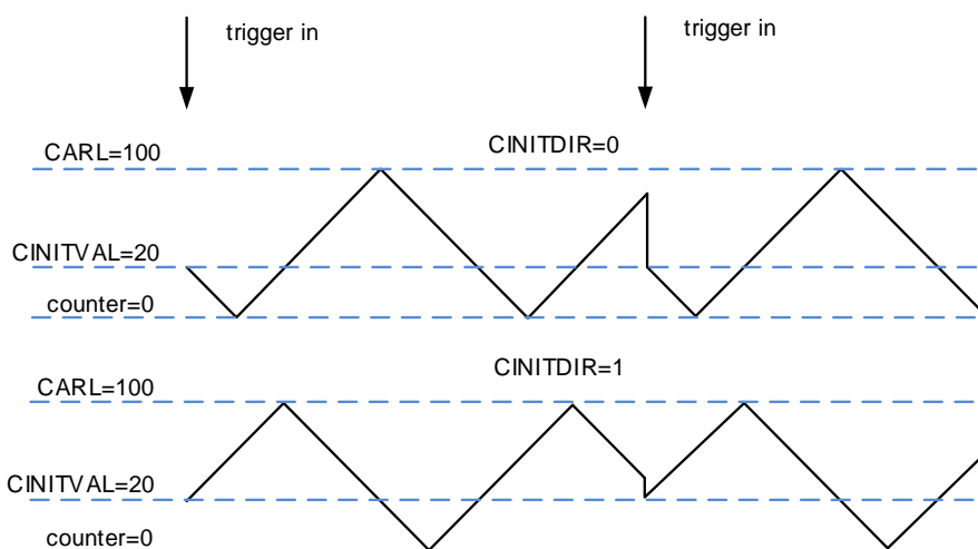
Figure 23-64. Direction of the counter after the reset in center-aligned counting mode
