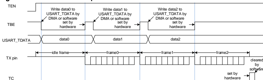
Figure 27-3. USART transmit procedure
