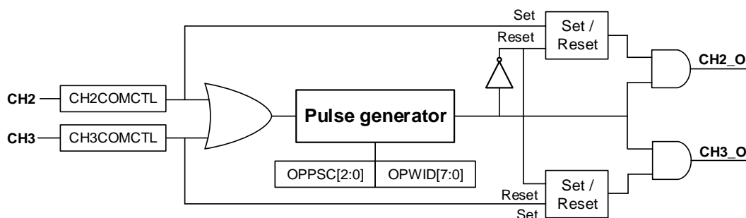
Figure 23-54. Programmable pulse output circuitry
