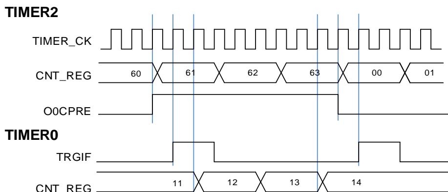
Figure 23-60. Pause mode of TIMER0 controlled by O0CPRE signal of TIMER2
