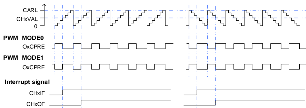
Figure 23-77. Timing chart of CAPWM
