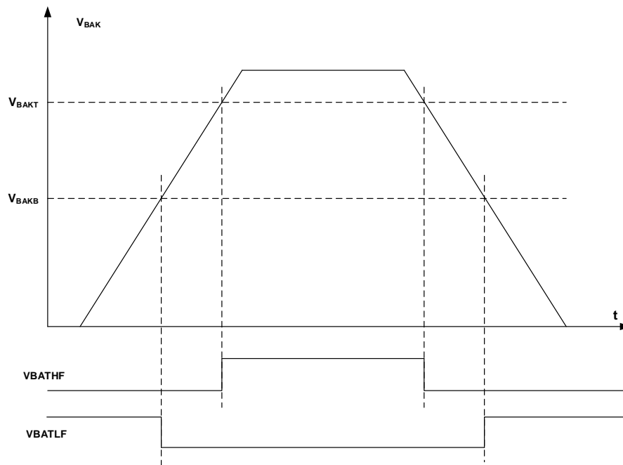
Figure 3-2. Waveform of the Backup domain voltage thresholds
