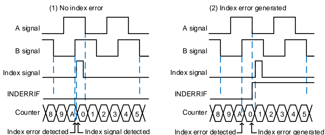
Figure 23-46. The Index error detection in up counting mode
