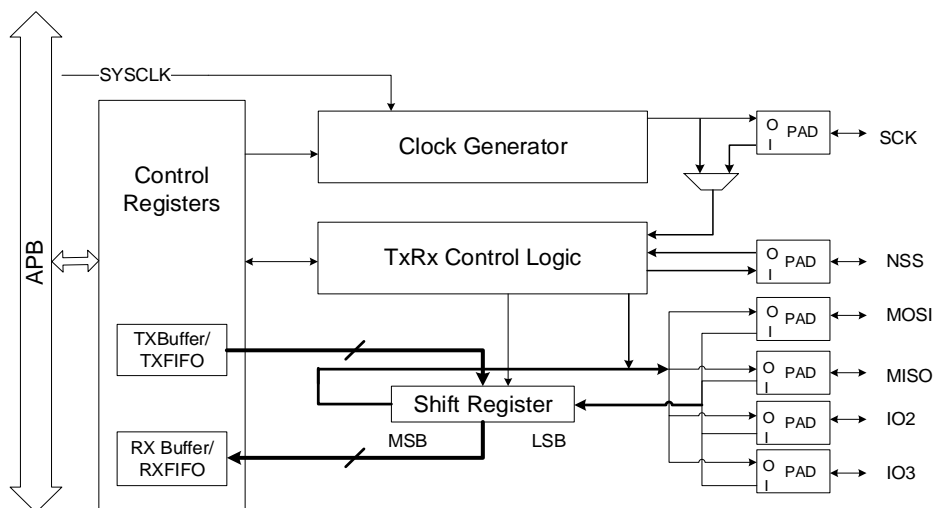
Figure 30-1. Block diagram of SPI
