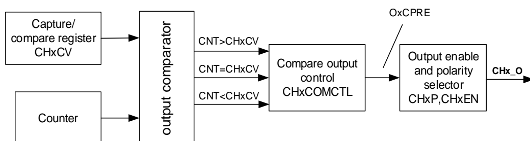
Figure 23-74. Output compare logic (x=0,1,2,3)
