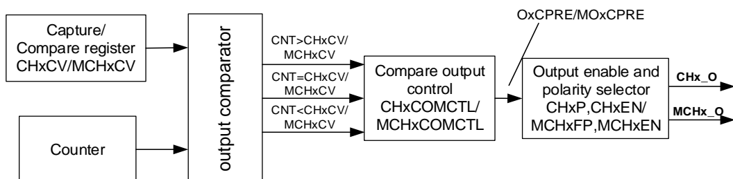
Figure 23-103. Output compare logic (when MCHxMSEL = 2'b11, x=0)
