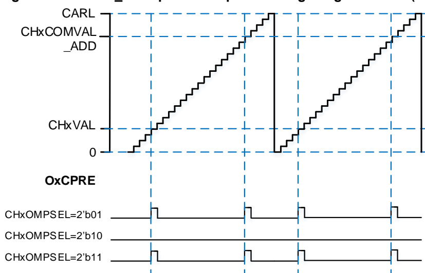
Figure 23-87. CHx_O output with a pulse in edge-aligned mode (CHxOMPSEL#2'b00)
