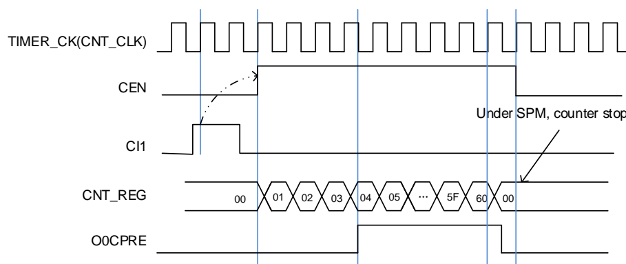
Figure 23-52. Single pulse mode TIMERx_CHxCV=0x04 , TIMERx_CAR=0x60
