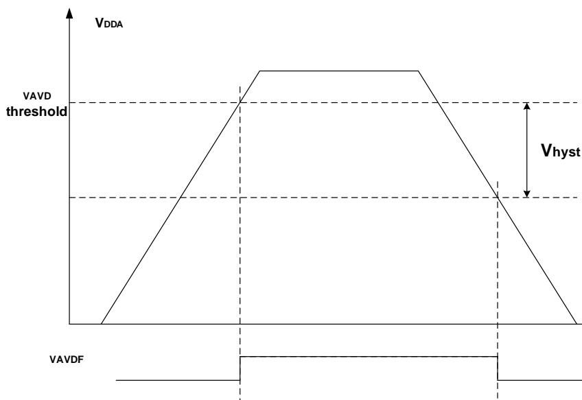
Figure 3-7. Waveform of the VAVD threshold
