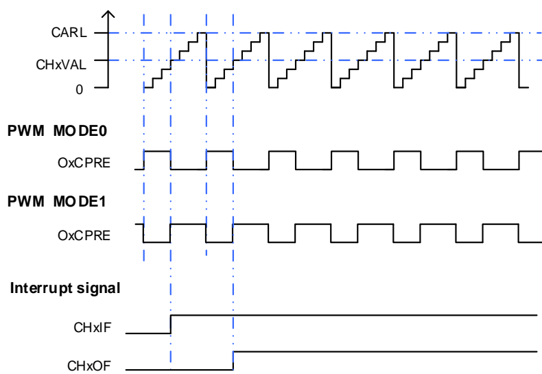
Figure 23-136. PWM mode timechart
