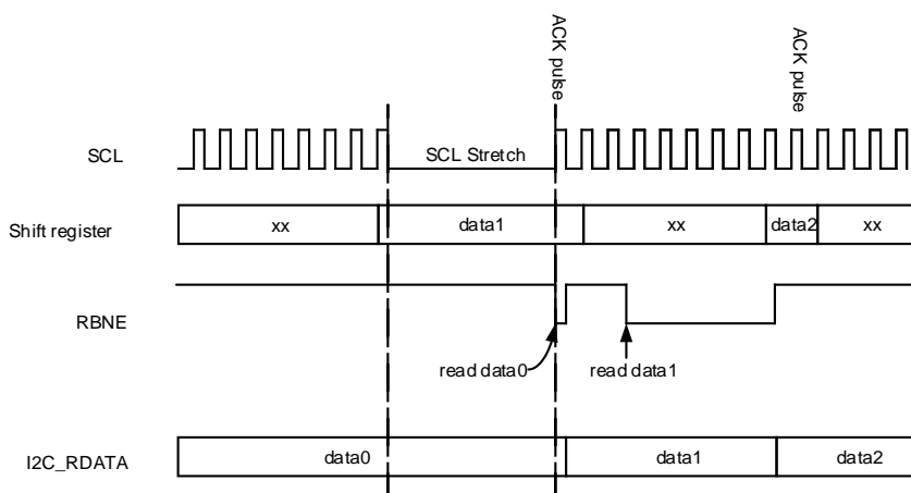
Figure 28-12. Data reception
