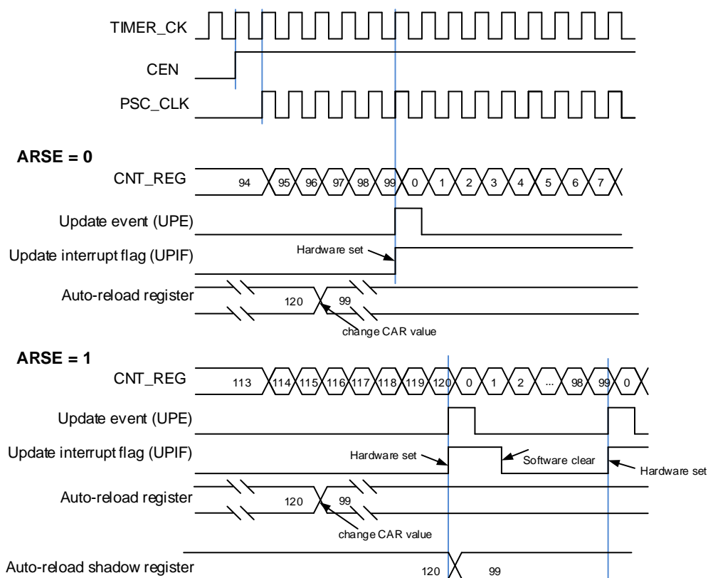
Figure 23-98. Timing diagram of up counting mode, change TIMERx_CAR on the go
