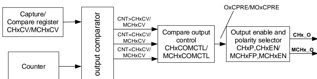
Figure 23-133. Output compare logic (when MCHxMSEL = 2'b00, x=0)
