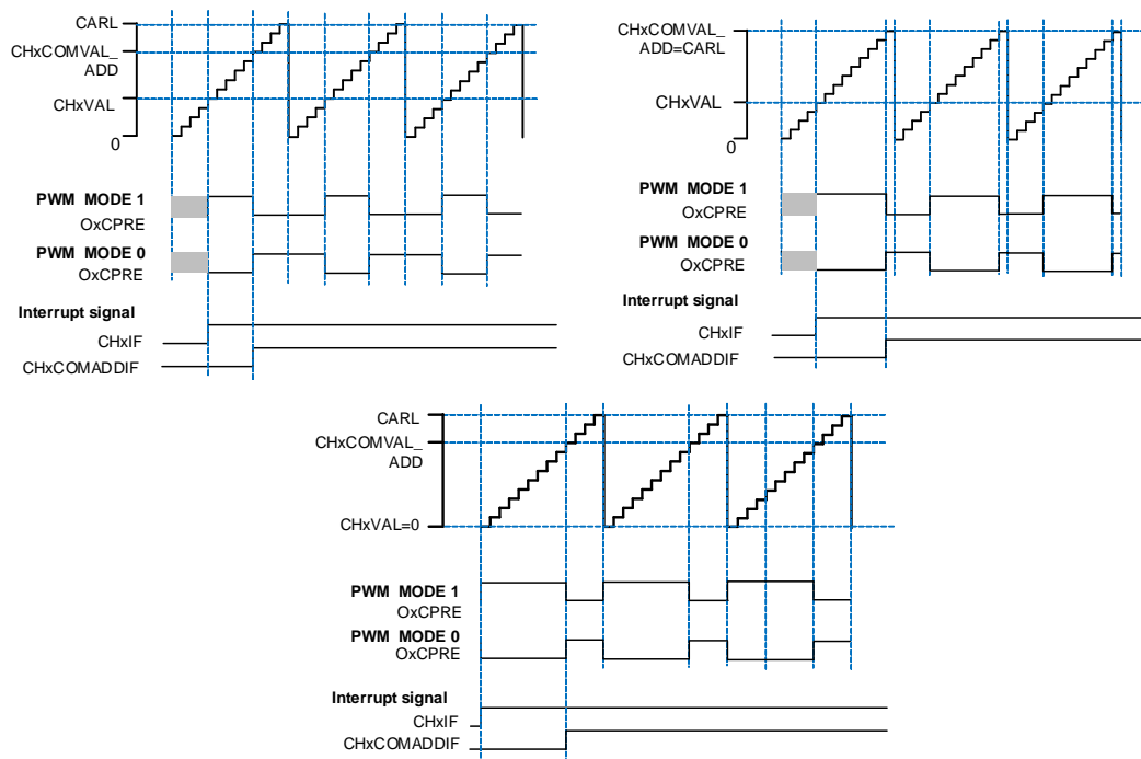
Figure 23-22. Channel x output PWM with (CHxVAL < CHxCOMVAL_ADD)
