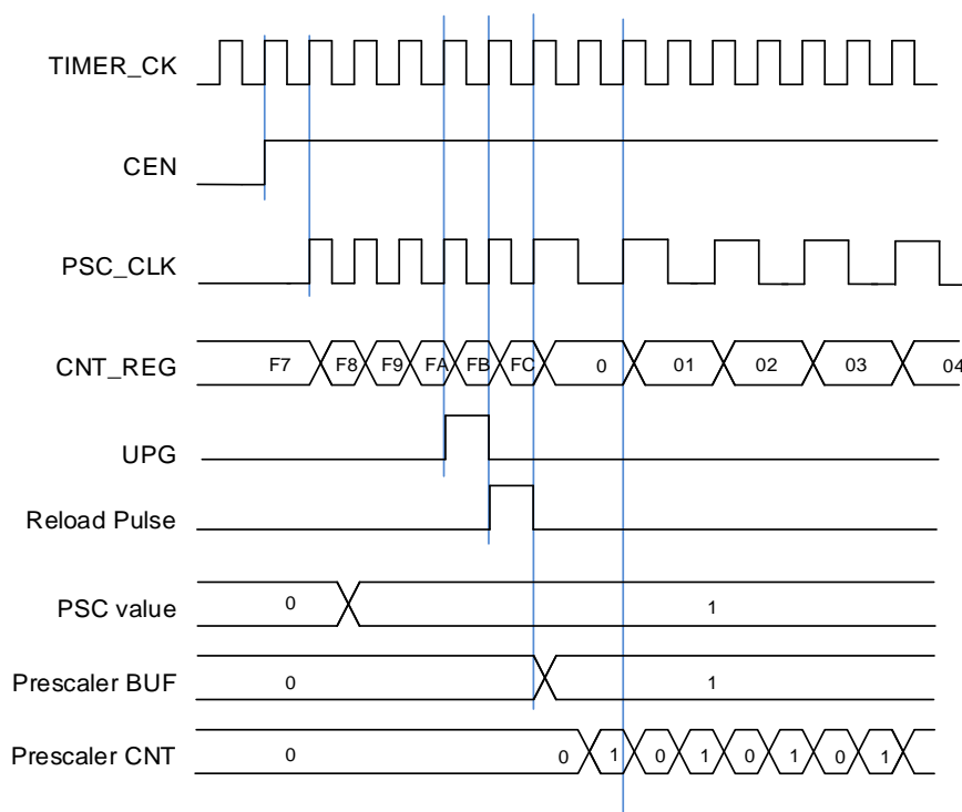
Figure 23-67. Counter timing diagram with prescaler division change from 1 to 2
