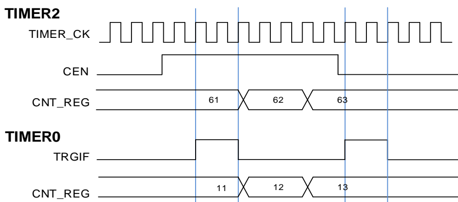
Figure 23-59. Pause mode of TIMER0 controlled by enable signal of TIMER2
