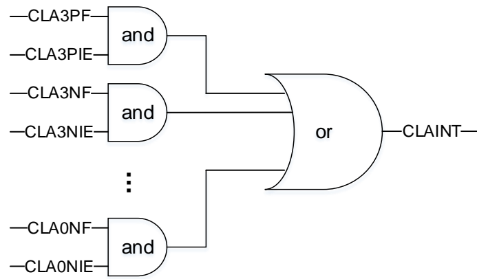
Figure 11-2. CLA interrupt logic
