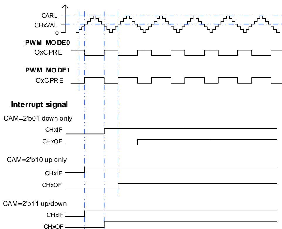
Figure 23-77. Timing chart of CAPWM
