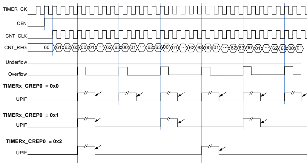
Figure 23-99. Repetition timechart for up-counter
