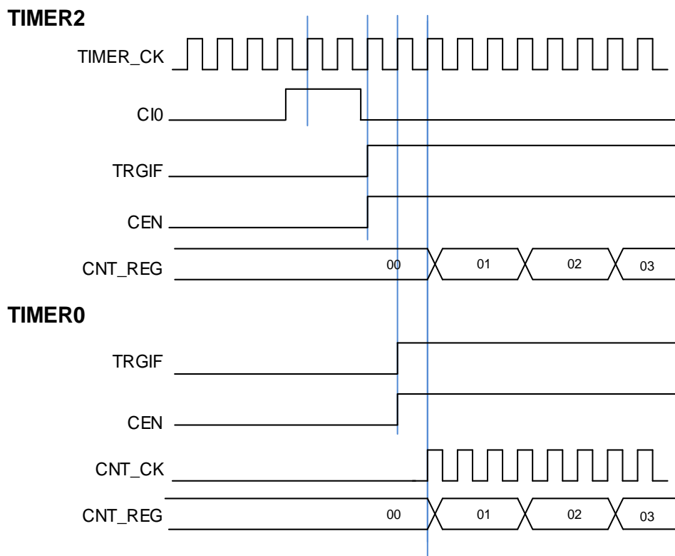
Figure 23-61. Trigger TIMER0 and TIMER2 by the CI0 signal of TIMER2
