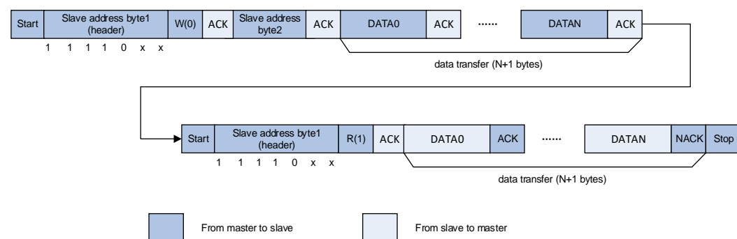
Figure 28-8. I2C communication flow with 10-bit address (Master Receive when HEAD10R=1)
