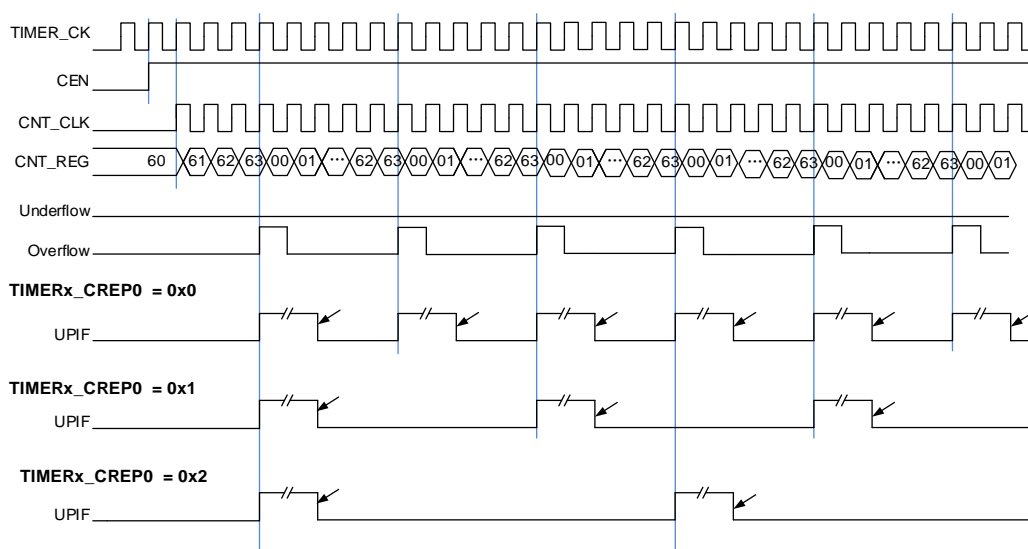
Figure 23-130. Repetition timechart for up-counter
