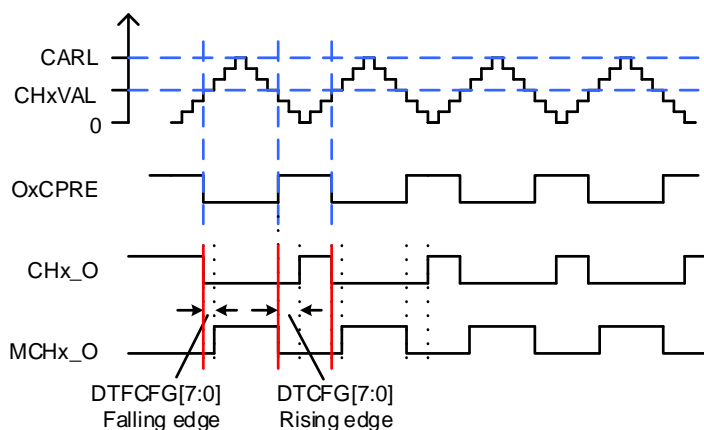
Figure 23-138. Complementary output with different dead time(DTDIFEN=1)
