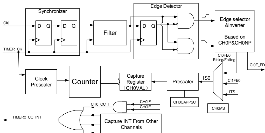
Figure 23-73. Input capture logic
