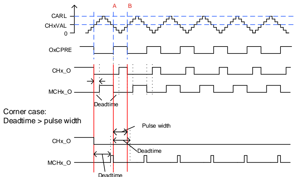
Figure 23-30. Complementary output with dead time insertion
