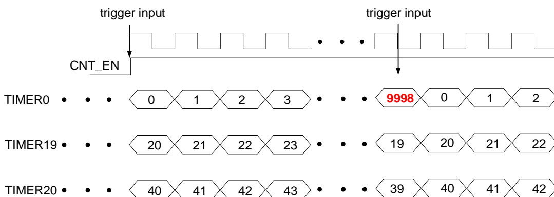
Figure 23-63. Phase shift diagram for three timers
