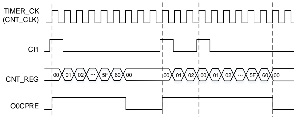
Figure 23-124. delayable single pulse mode TIMERx_CHxCV=0x00, TIMERx_CAR=0x60
