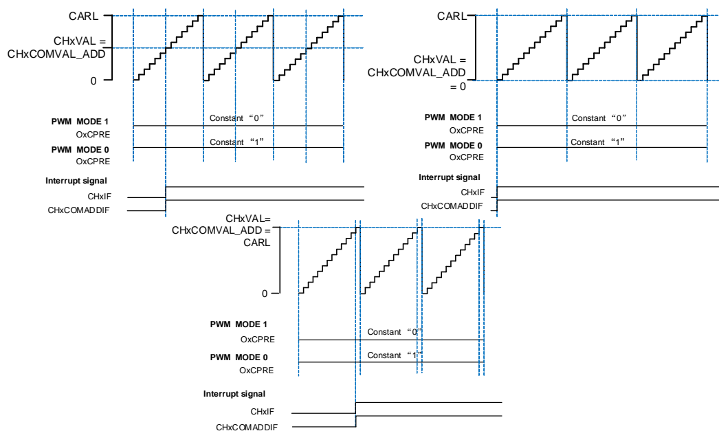
Figure 23-82. Channel x output PWM with (CHxVAL = CHxCOMVAL_ADD)
