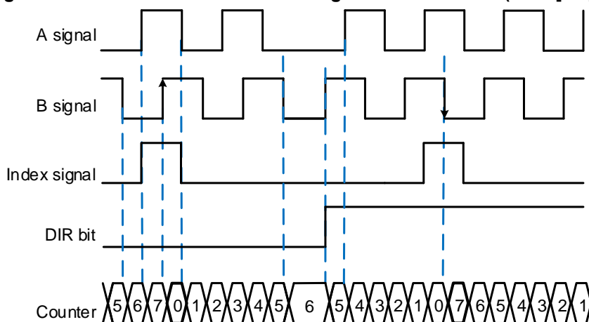
Figure 23-43. Counter with the index signal the same as A ( INDP[1:0]=2'b11 )
