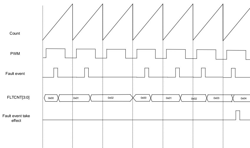
Figure 25-52. Fault counter when FLTxRSTM bit is 1 and FLTxCNT[2:0] = 0x03
