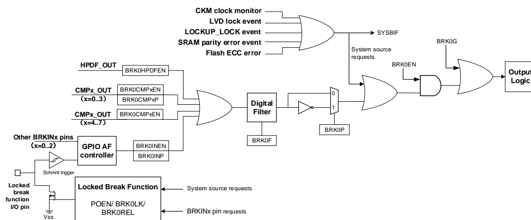
Figure 23-36. BRKINx (x=0...2) pins logic with BREAK0 function
