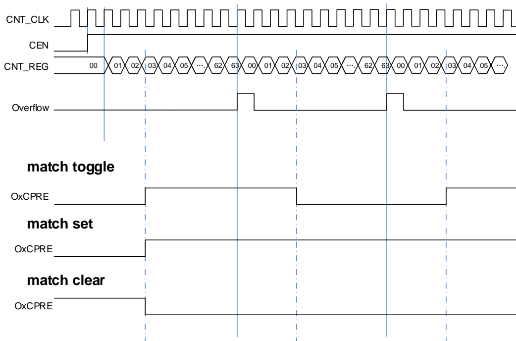
Figure 23-75. Output-compare under three modes
