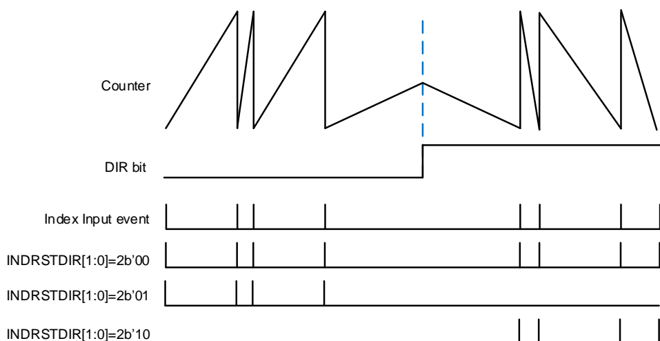
Figure 23-44. The relationship between the index signal and counter reset events
