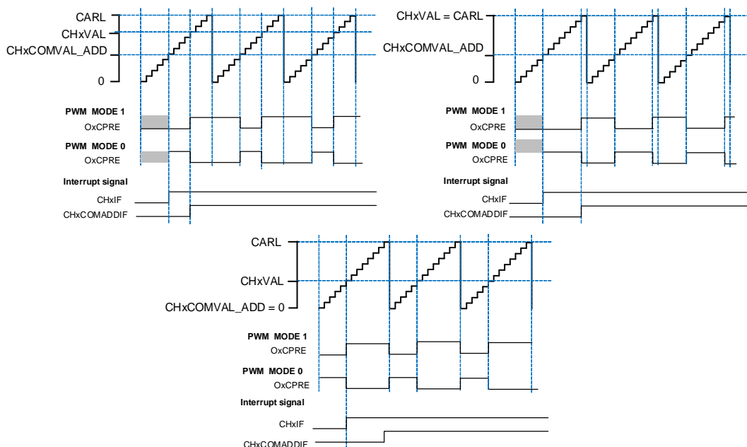
Figure 23-24. Channel x output PWM with ( CHxVAL > CHxCOMVAL\_ADD )
