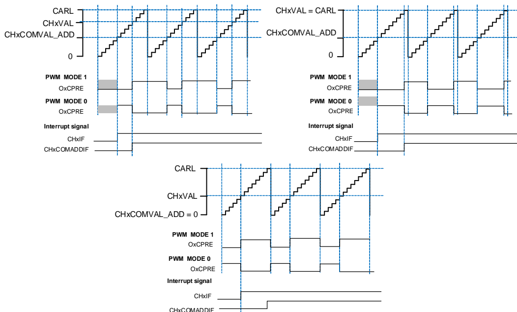
Figure 23-111. Channel x output PWM with (CHxVAL > CHxCOMVAL_ADD)
