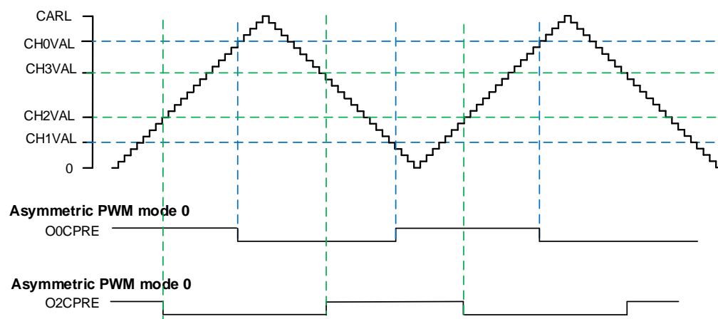
Figure 23-80. CH0 and CH2 with asymmetric PWM mode
