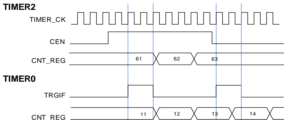
Figure 23-57. Trigger mode of TIMER0 controlled by enable signal of TIMER2
