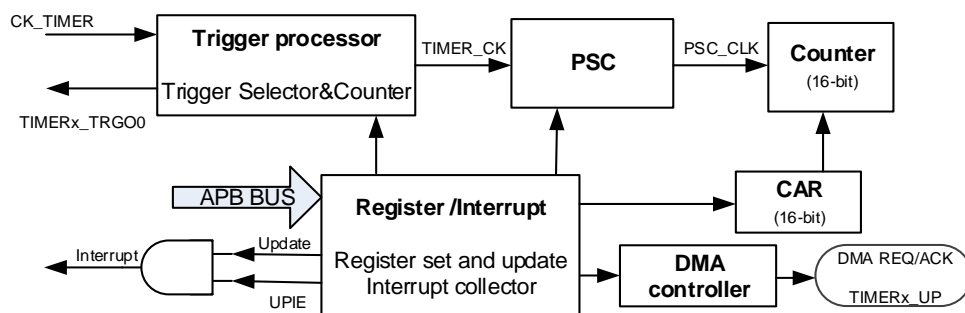
Figure 23-143. Basic timer block diagram
