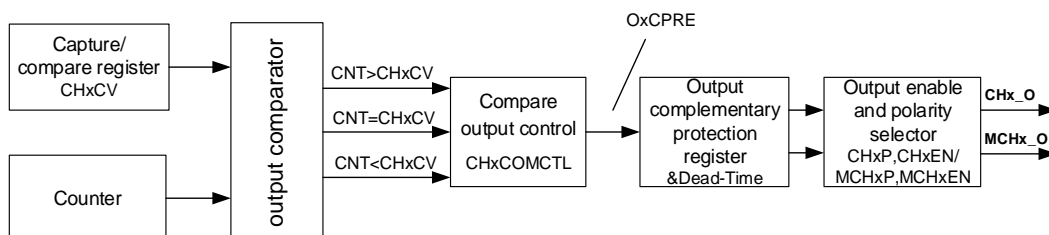
Figure 23-134. Output compare logic (when MCHxMSEL = 2'b11, x=0)
