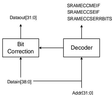
Figure 1-3. ECC decoder
