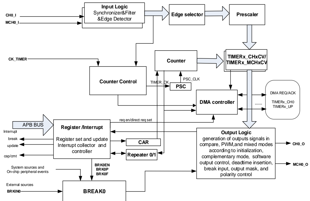
Figure 23-125. General level4 timer block diagram
