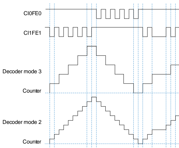
Figure 23-41. Example of counter operation in decoder mode 2 / 3 (CH0P / CH1P=0)
