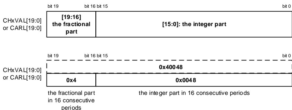
Figure 23-107. Adjustment mode: Data format and the register bit-field
