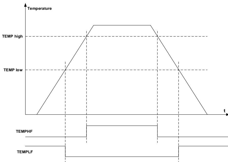
Figure 3-3. Temperature thresholds
