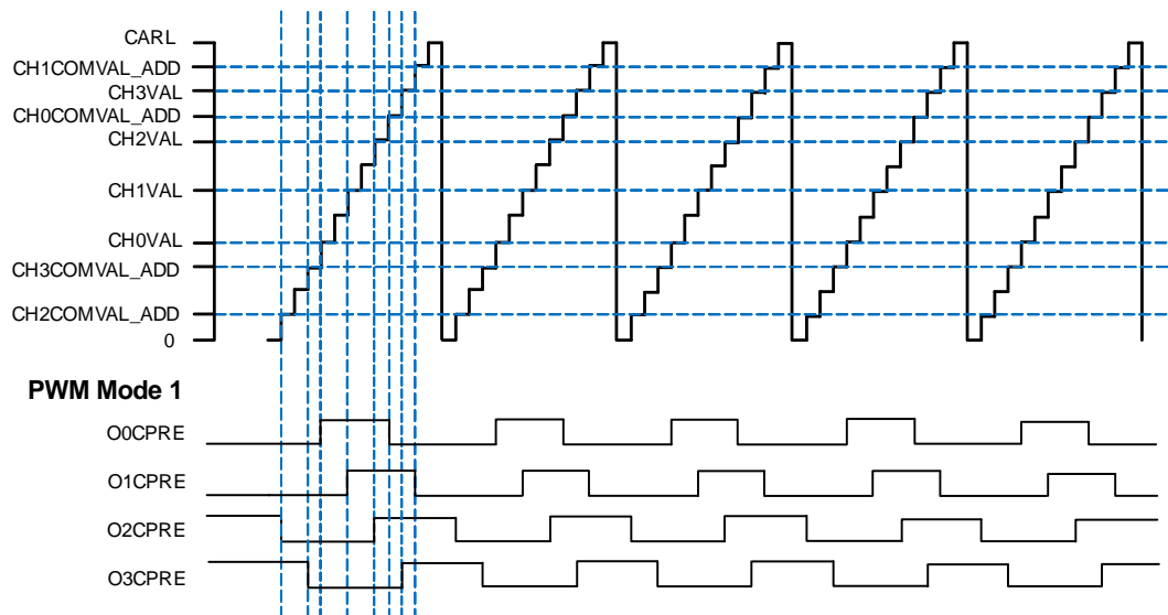
Figure 23-86. Four Channels outputs in Composite PWM mode
