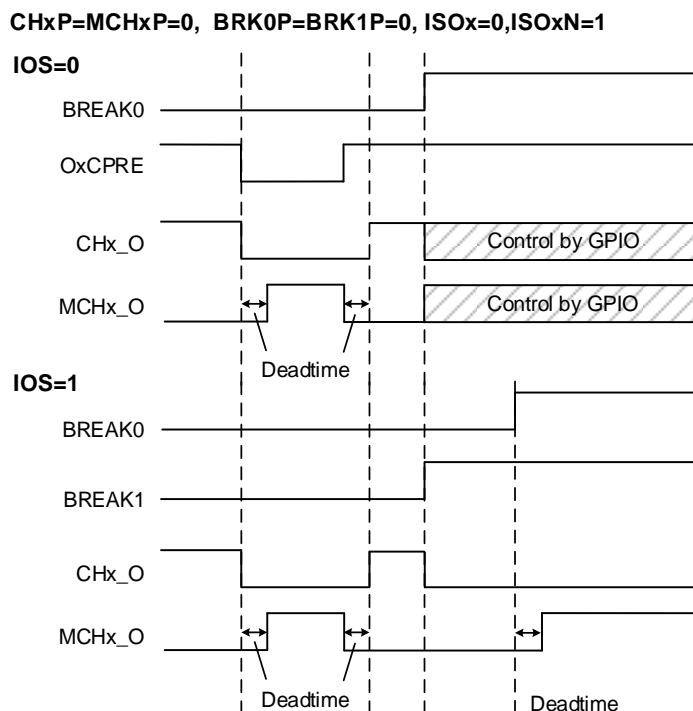
Figure 23-35. Output behavior of the channel outputs with the BREAK0 and BREAK1
