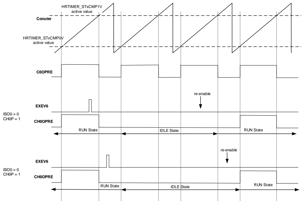
Figure 25-36. ISO0 = 0 and CHOP = 1 in delayed IDLE
