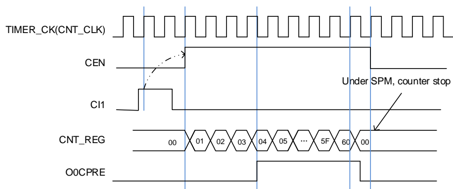
Figure 23-123. Single pulse mode TIMERx\_CHxCV = 0x04 TIMERx\_CAR=0x60
