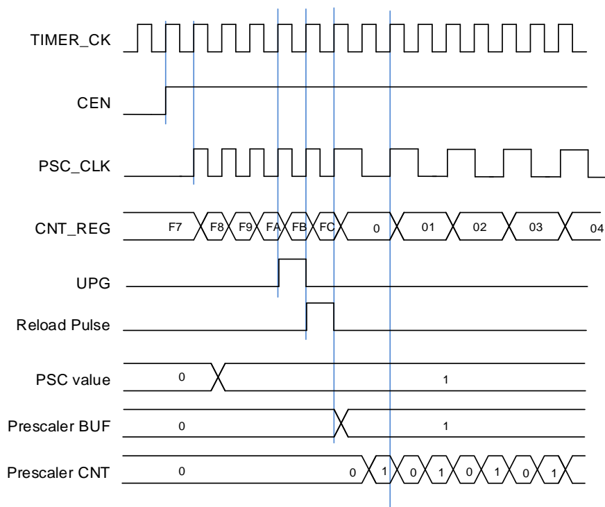
Figure 23-127. Counter timing diagram with prescaler division change from 1 to 2
