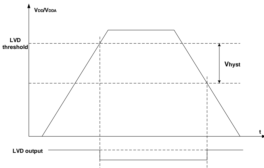
Figure 3-6. Waveform of the LVD threshold
