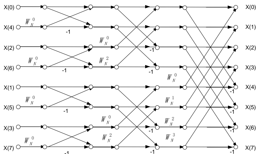
Figure 15-2 8 point DIT FFT flow digram
