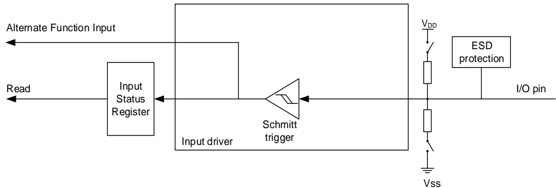
Figure 7-2. Input configuration
