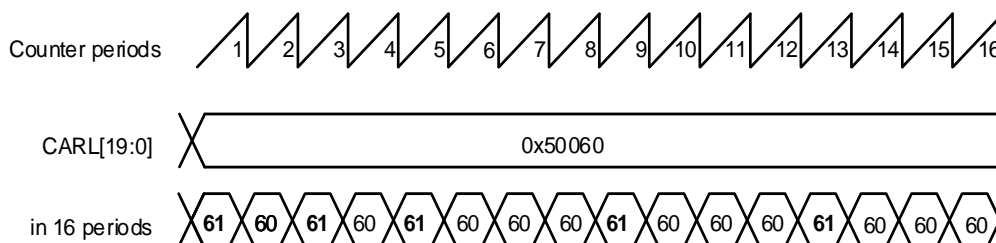
Figure 23-149. Adjustment mode schematic diagram
