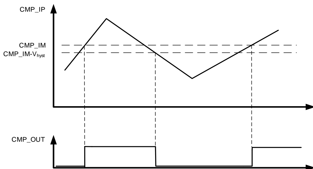
Figure 19-2. CMP hysteresis
