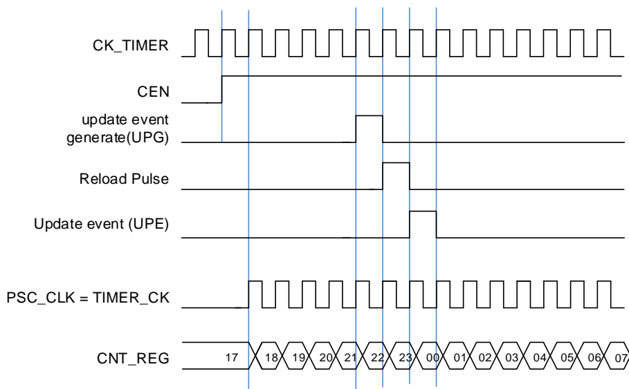
Figure 23-144. Normal mode, internal clock divided by 1
