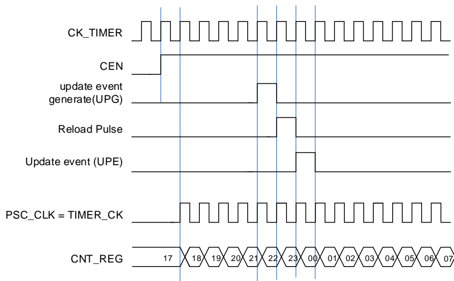
Figure 23-126. Normal mode, internal clock divided by 1
