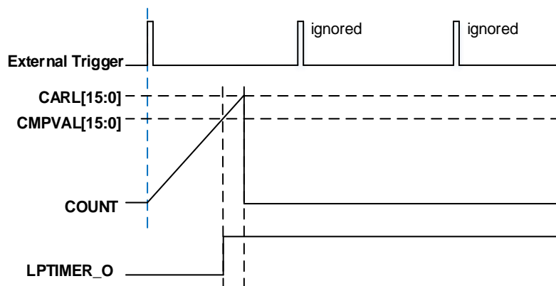
Figure 24-7. LPTIMER output with OMSEL = 1(16-bit)
