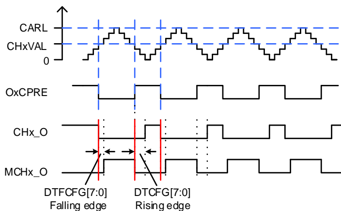
Figure 23-31. Complementary output with different dead time(DTDIFEN=1)
