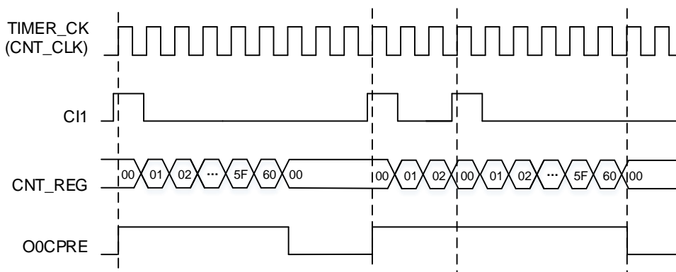
Figure 23-93. delayable single pulse mode TIMERx_CHxCV=0x00, TIMERx_CAR=0x60
