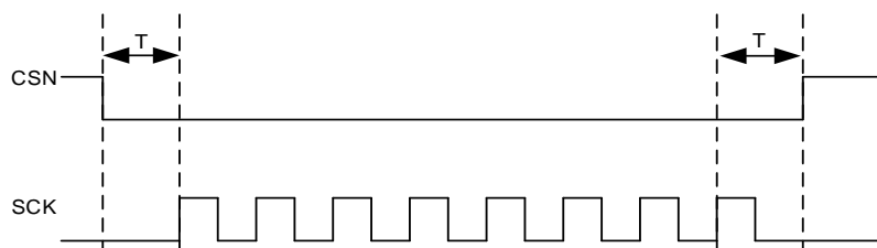
Figure 31-5 Behavior of CSN and SCK (CSNCKM = 0)
