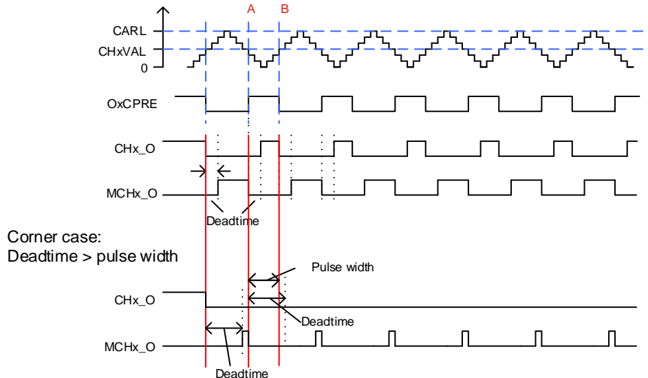
Figure 23-115. Complementary output with dead-time insertion
