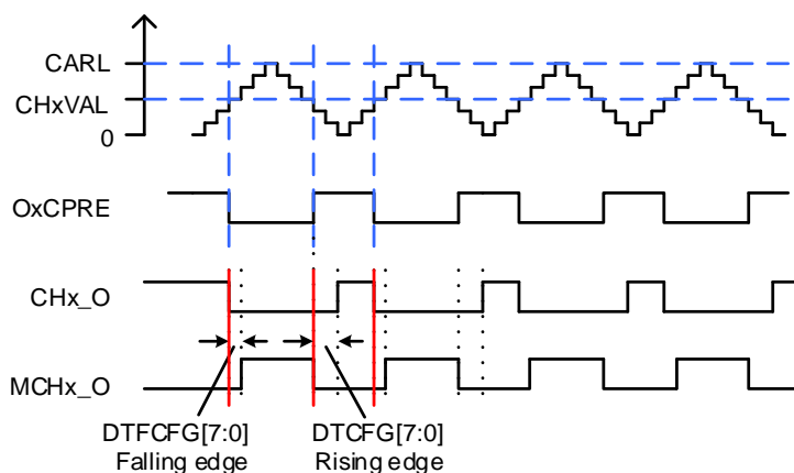
Figure 23-116. Complementary output with different dead time(DTDIFEN=1)
