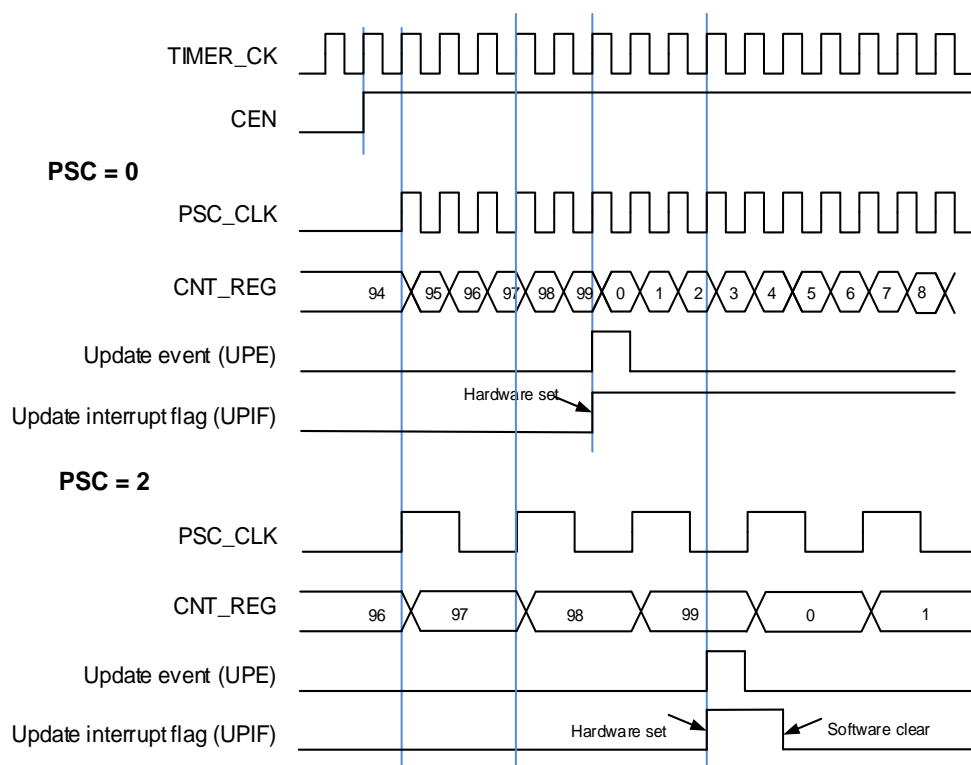
Figure 23-97. Timing diagram of up counting mode, PSC=0 / 2
