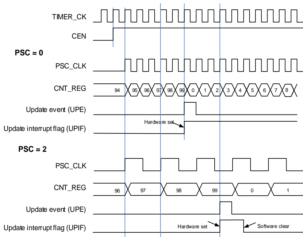
Figure 23-128. Timing diagram of up counting mode, \text{PSC}=0/2
