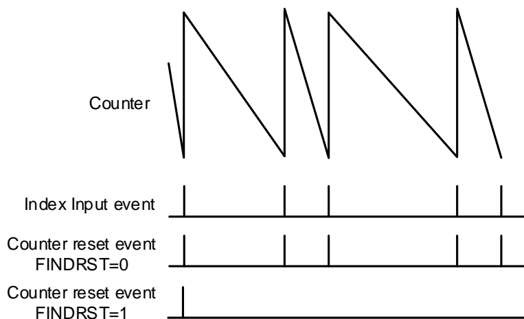
Figure 23-45. The counter reset events with the FINDRST bit
