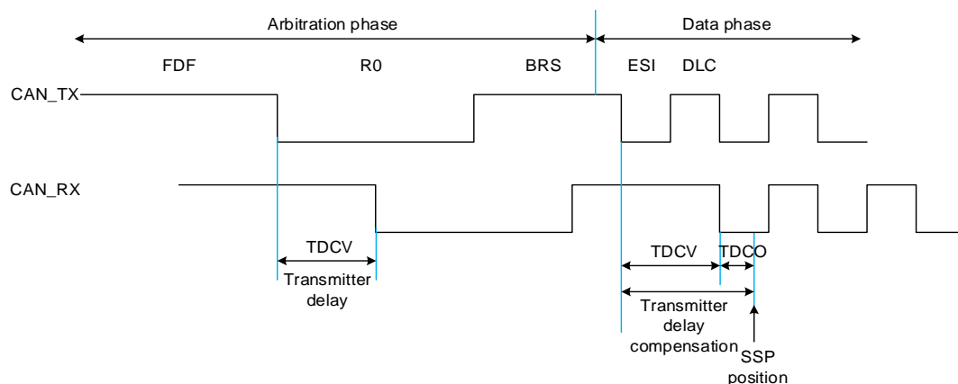
Figure 29-2. Transmitter delay
