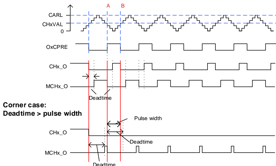
Figure 23-137. Complementary output with dead-time insertion
