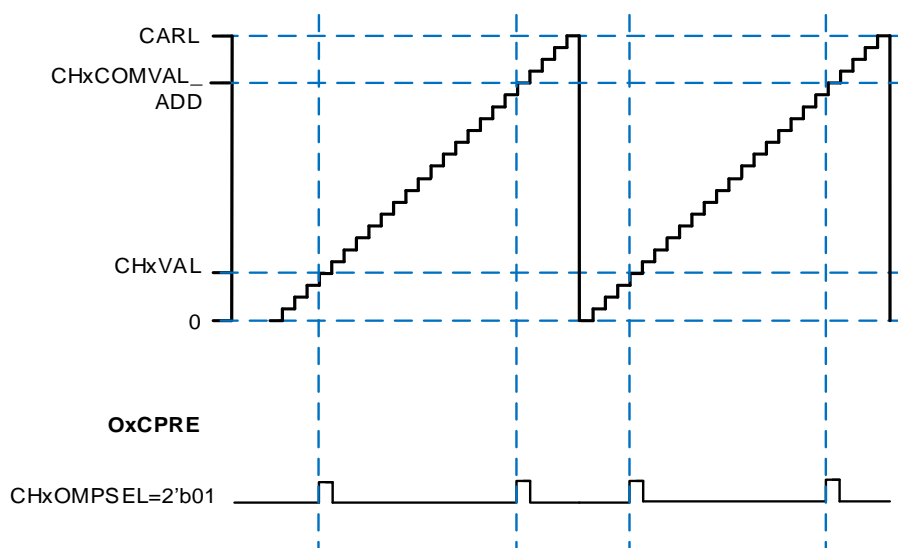
Figure 23-114. CHx_O output with a pulse in edge-aligned mode (CHxOMPSEL = 2'b00)
