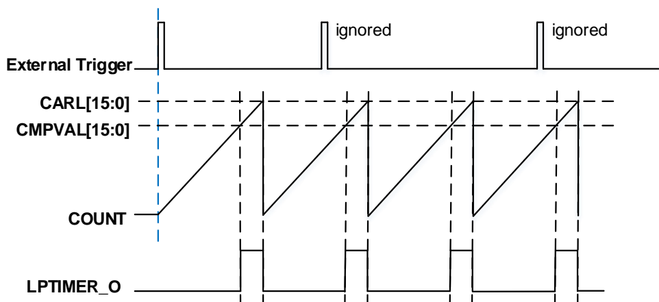
Figure 24-8. LPTIMER output with CTNMST = 1(16-bit)
