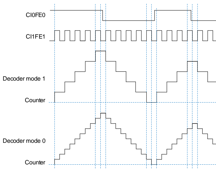
Figure 23-40. Example of counter operation in decoder mode 0 / 1 with CH1P=0
