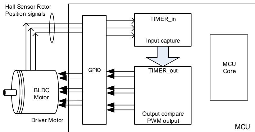
Figure 23-47. Hall sensor is used for BLDC motor
