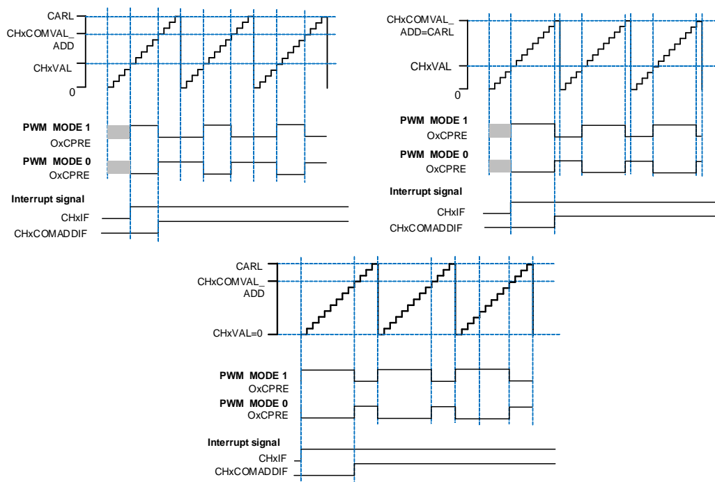
Figure 23-109. Channel x output PWM with (CHxVAL < CHxCOMVAL_ADD)
