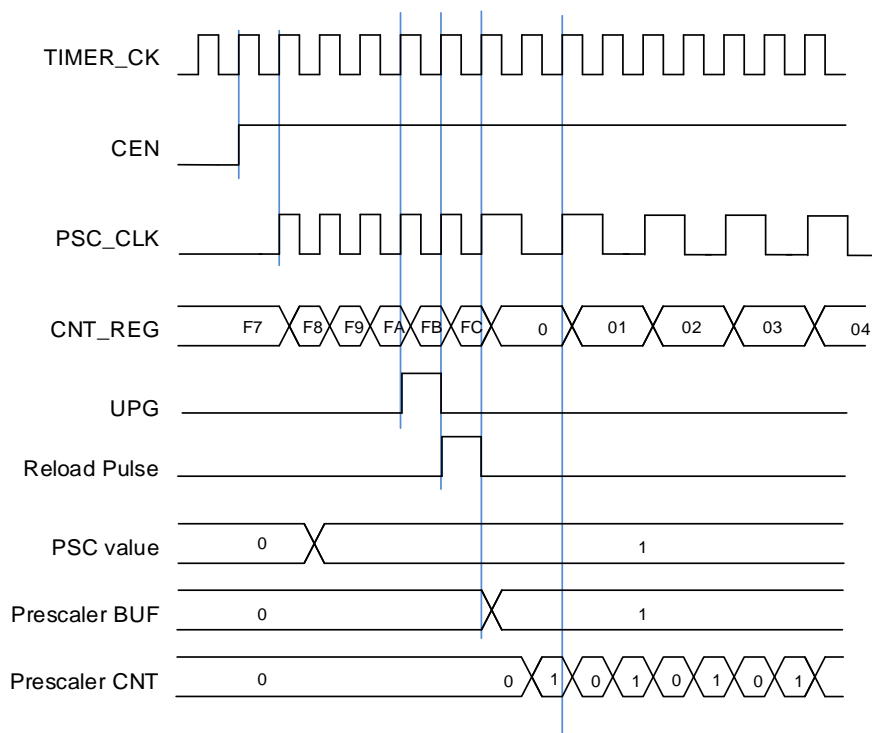
Figure 23-145. Counter timing diagram with prescaler division change from 1 to 2
