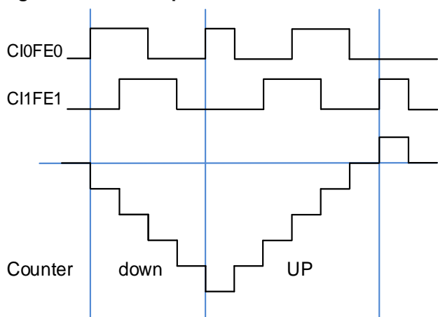
Figure 23-38. Example of decoder interface mode with CI0FE0 polarity inverted
