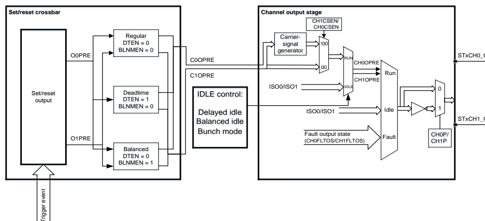
Figure 25-19. Channel output diagram
