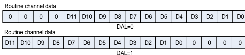
Figure 17-7. 12-bit Data storage mode
