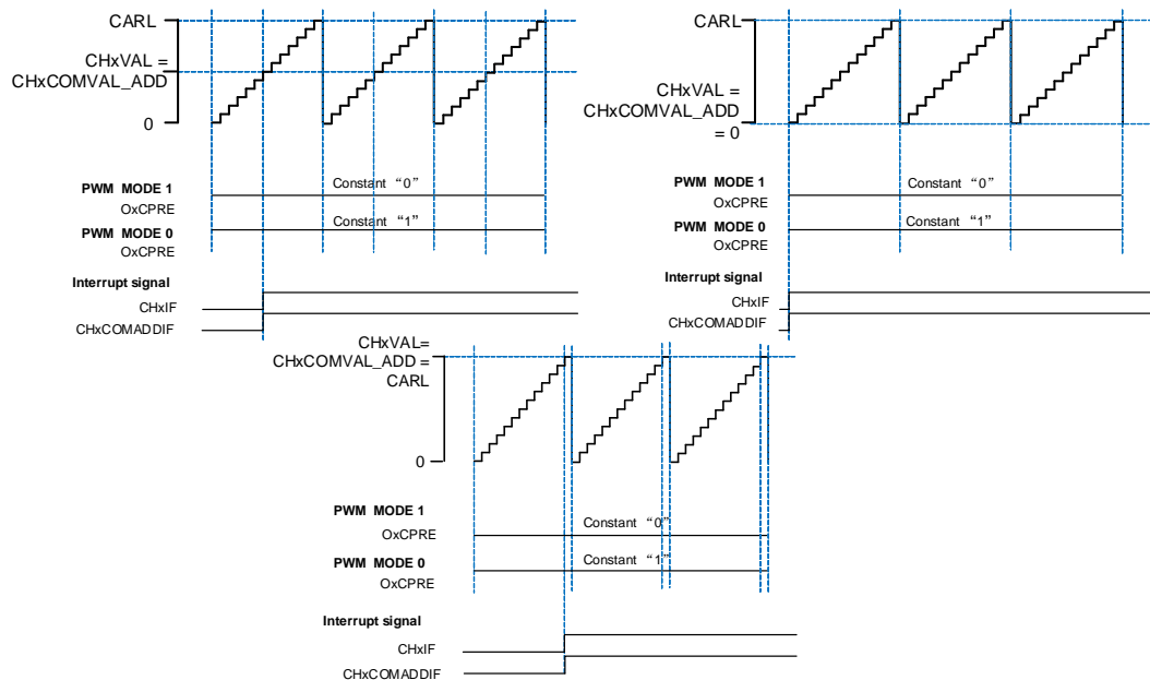
Figure 23-23. Channel x output PWM with ( CHxVAL = CHxCOMVAL\_ADD )
