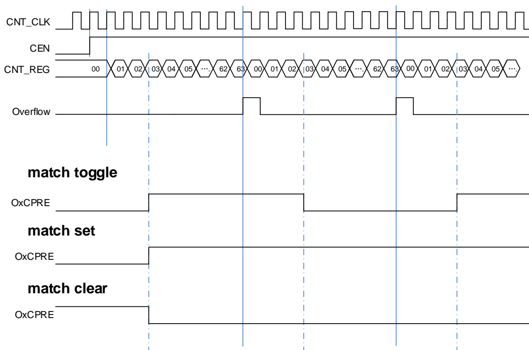
Figure 23-105. Output-compare in three modes
