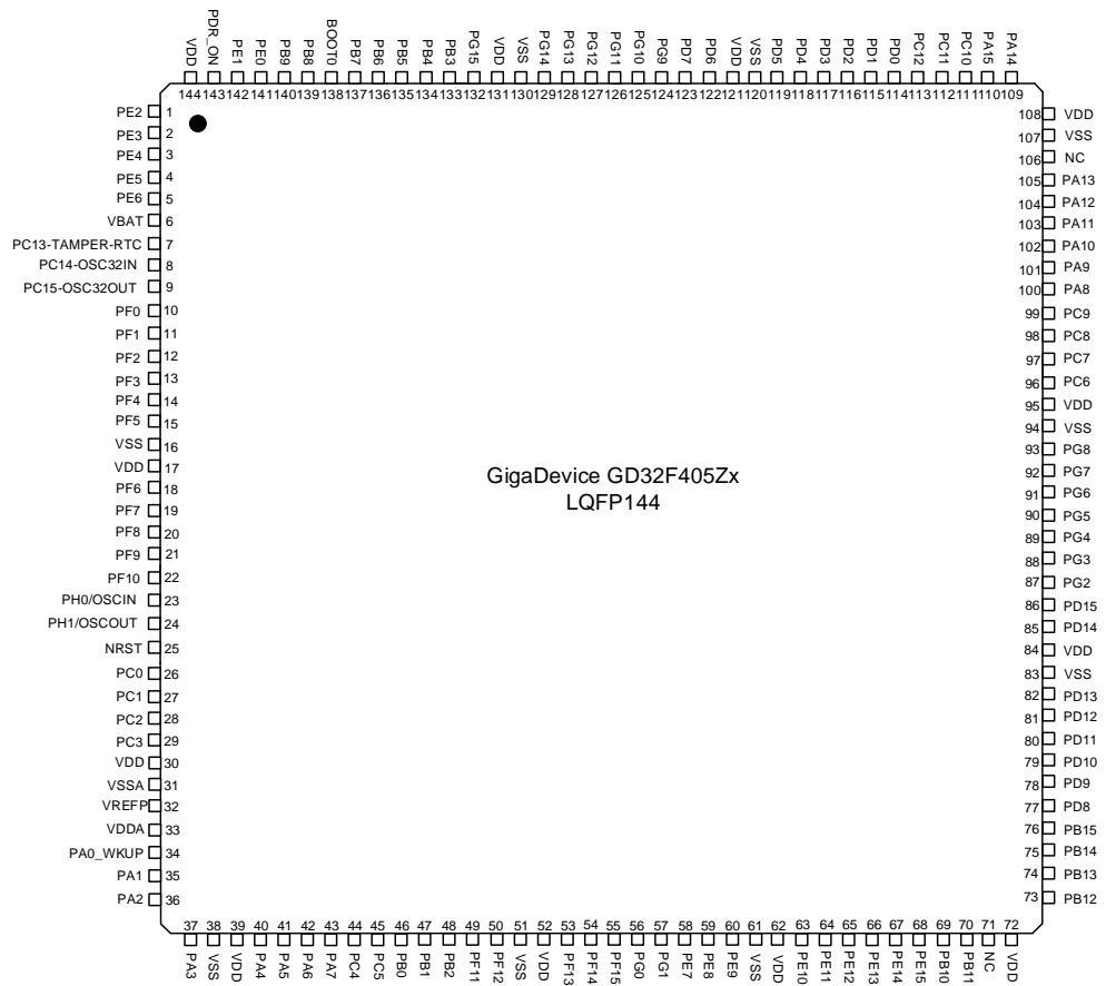
Figure 2-3. GD32F405Zx LQFP144 pinouts
