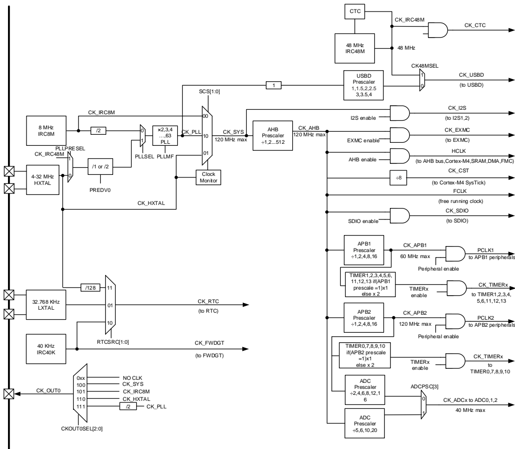
Figure 5-2. Clock tree
