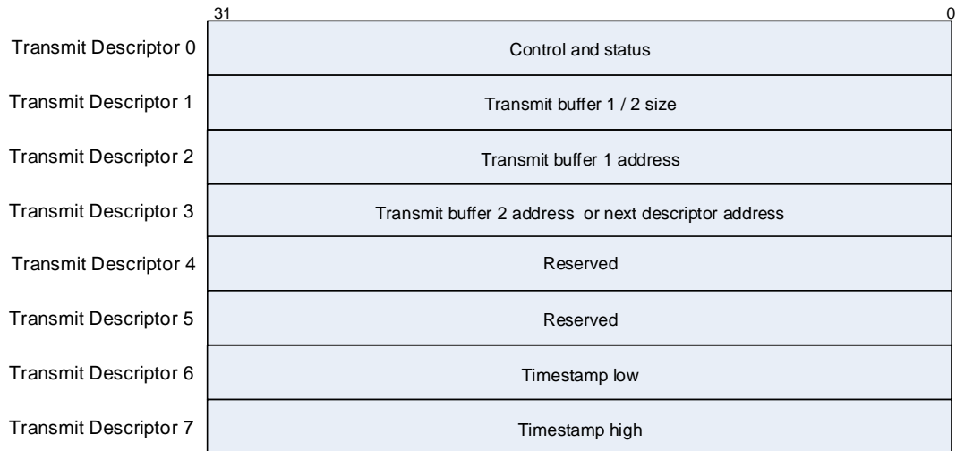
Figure 23-8. Transmit descriptor in enhanced mode
