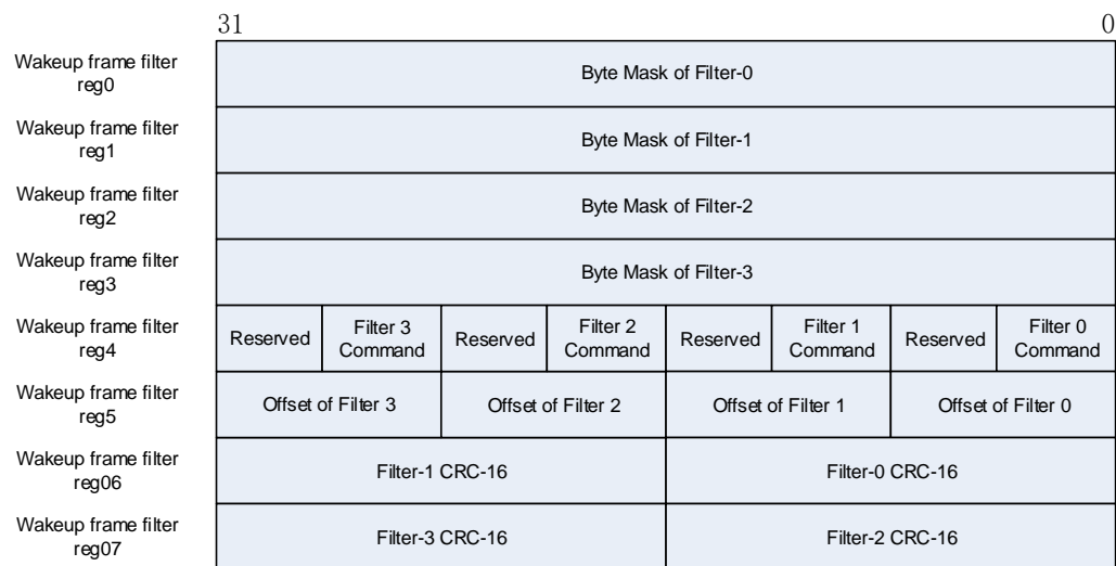
Figure 23-15. Wakeup frame filter register
