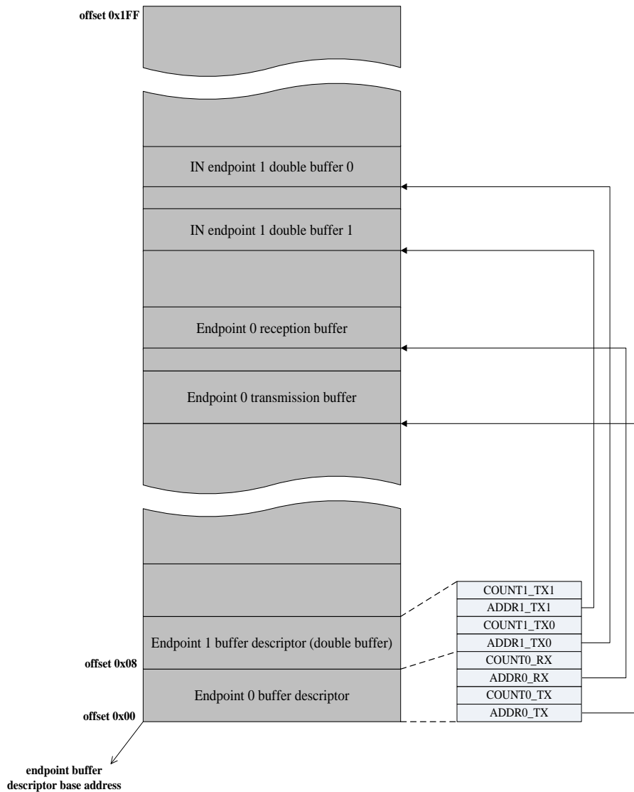
Figure 24-2. an example with buffer descriptor table usage (USB_BADDR = 0)
