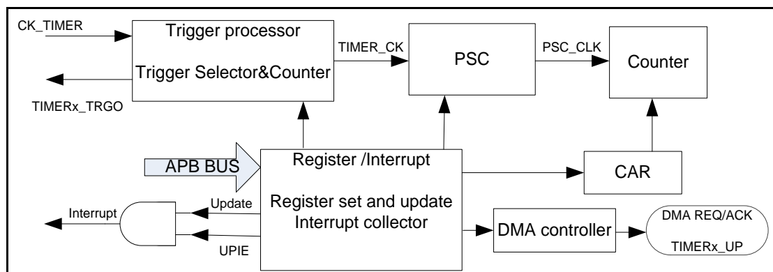
Figure 16-64. Basic timer block diagram
