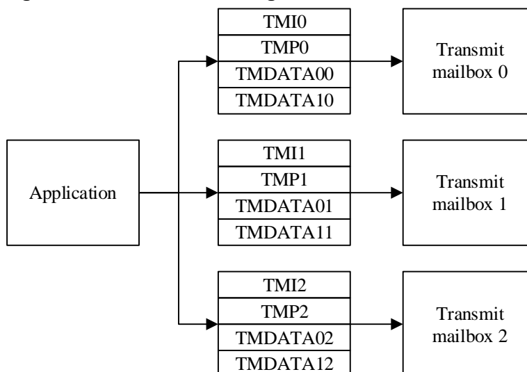
Figure 22-2. Transmission register
