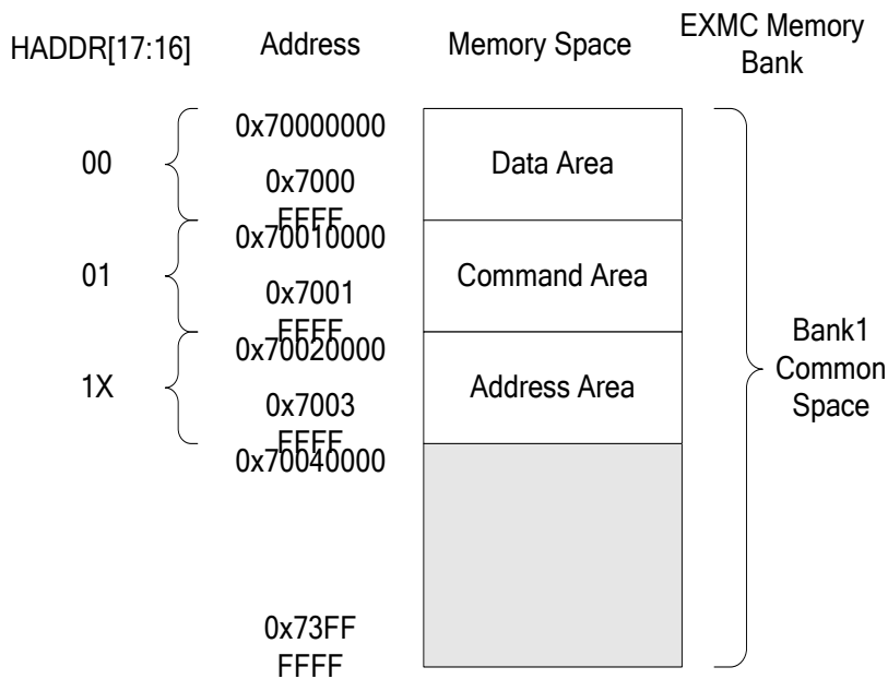
Figure 21-5. Diagram of bank1 common space
