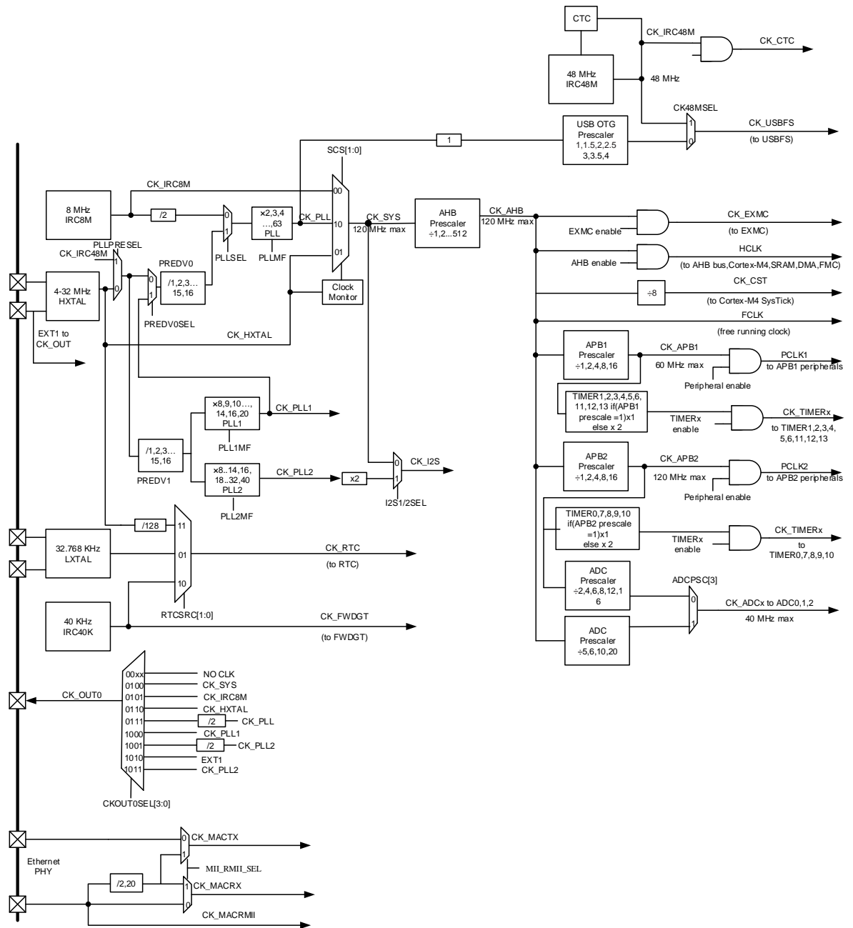
Figure 5-6. Clock tree
