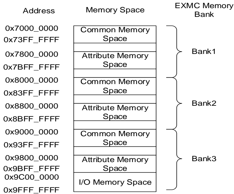
Figure 21-4. NAND/PC Card address mapping
