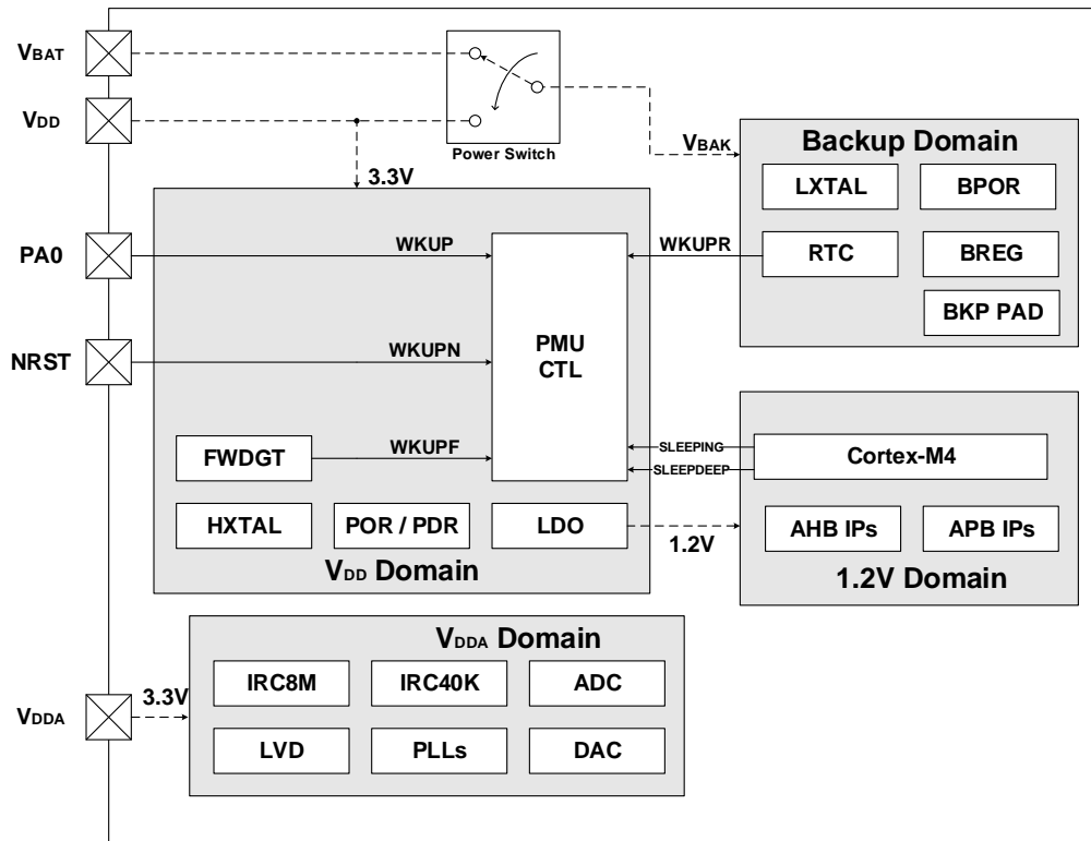
Figure 3-1. Power supply overview
