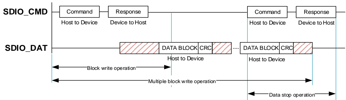
Figure 20-3. SDIO multiple blocks write operation
