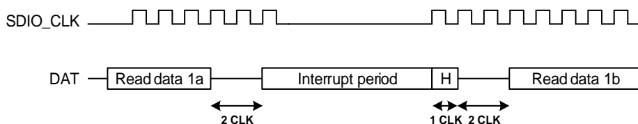
Figure 20-12. Read wait control by stopping SDIO_CLK
