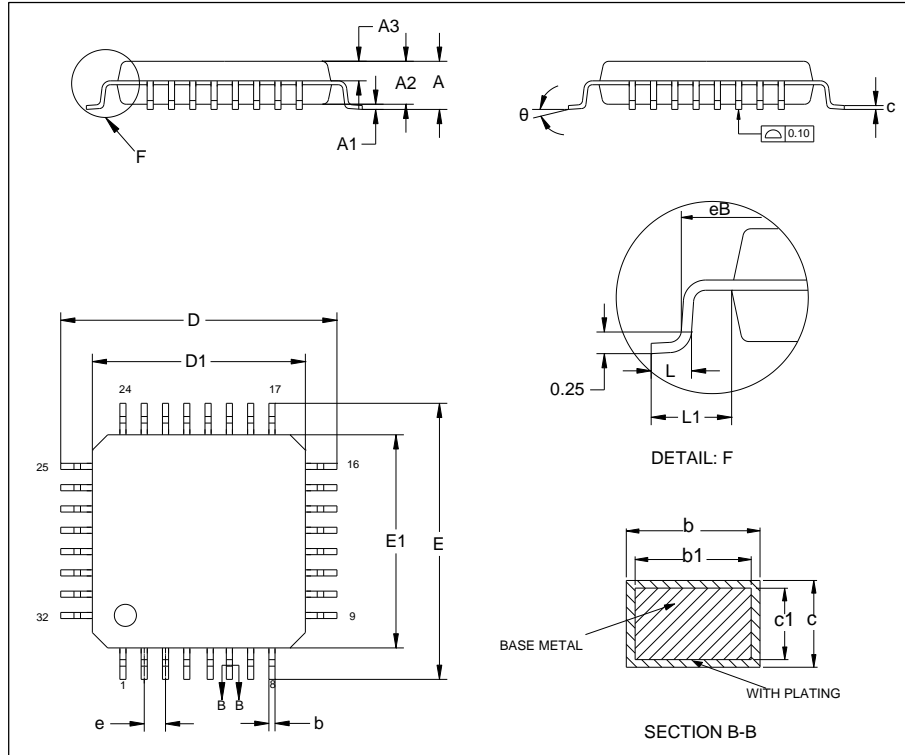
Figure 5-5. LQFP32 package outline
