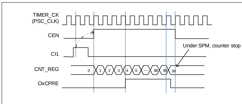
图 18-64. 单脉冲模式, TIMERx_CHxCV = 4 TIMERx_CAR=99
