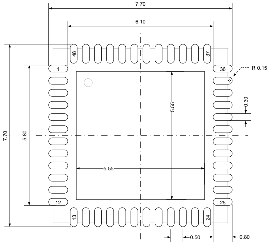
Figure 5-10. QFN48 recommended footprint
