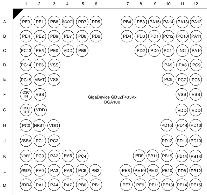
Figure 2-4. GD32F403Vx BGA100 pinouts
