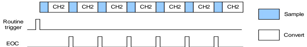
Figure 12-3. Continuous operation mode
