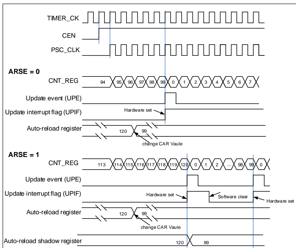
Figure 16-61. Timing chart of up counting mode, change TIMEx_CAR on the go
