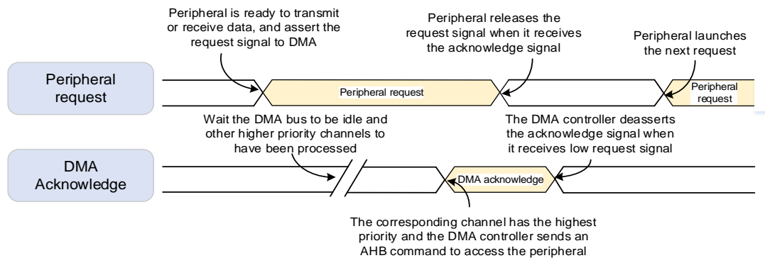
Figure 10-2. Handshake mechanism
