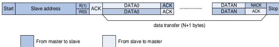
Figure 18-6. I2C communication flow with 7-bit address
