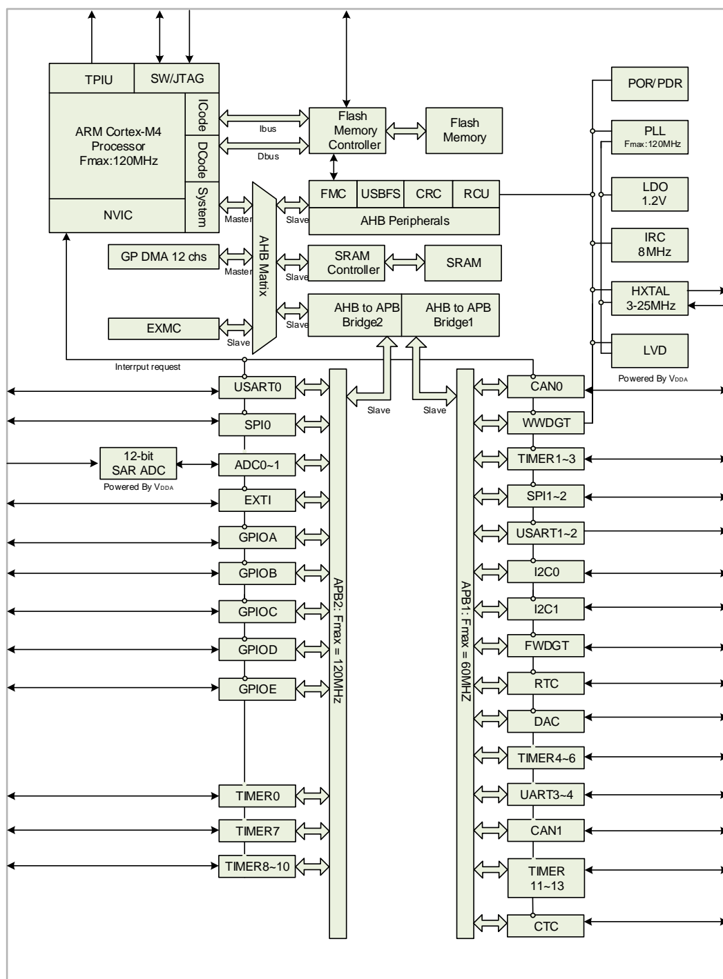
Figure 1-2. GD32C10x series system architecture
