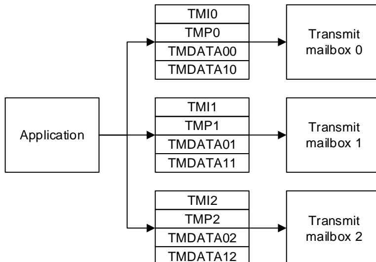
Figure 21-2. Transmission register
