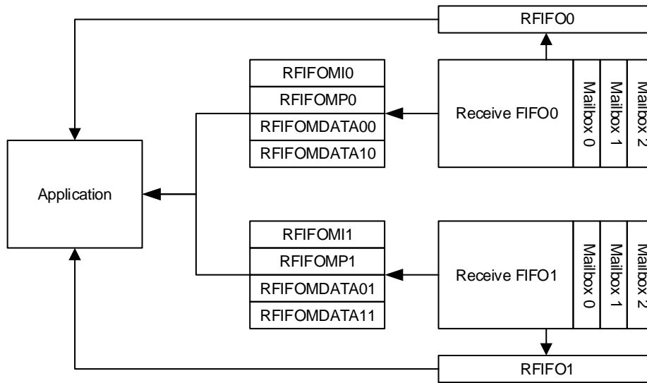
Figure 21-4. Reception register
