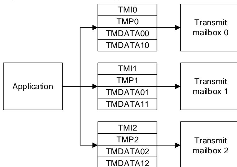
Figure 21-2. Transmission register
