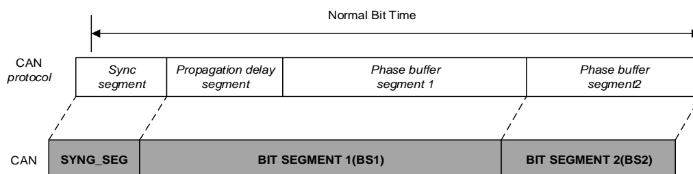
Figure 21-11. The bit time
