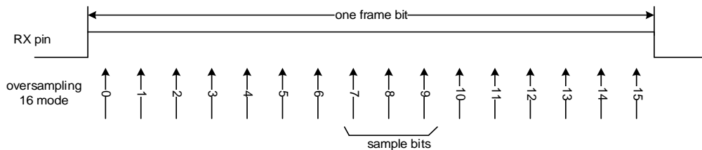
Figure 17-4. Receiving a frame bit by oversampling method
