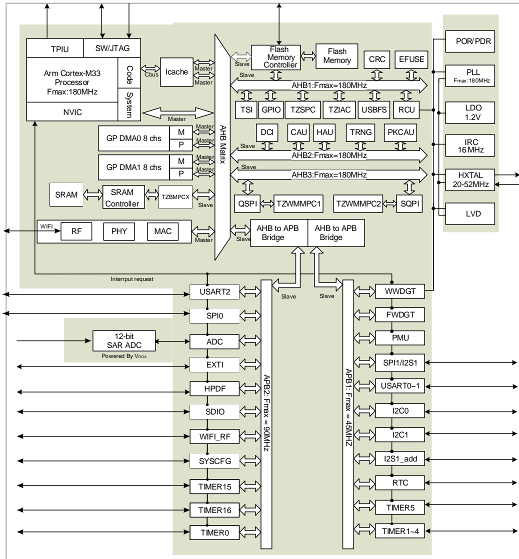
Figure 2-1. GD32W515xx block diagram
