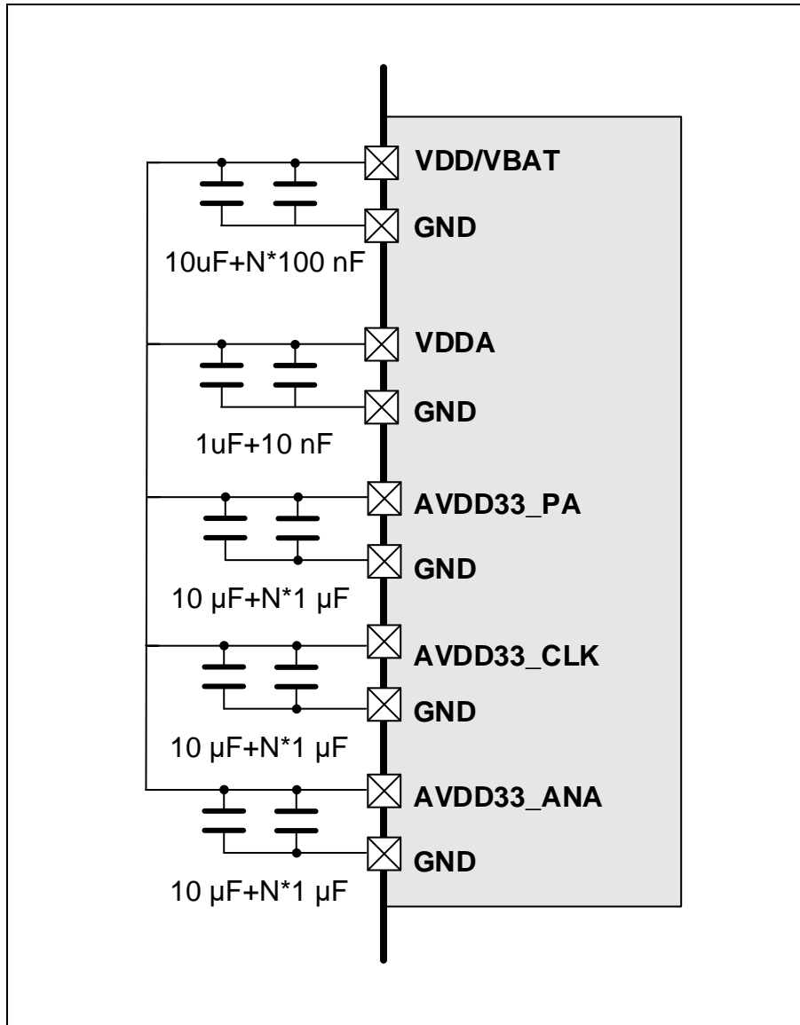
Figure 4-1. Recommended power supply decoupling capacitors (1)(2)(3)
