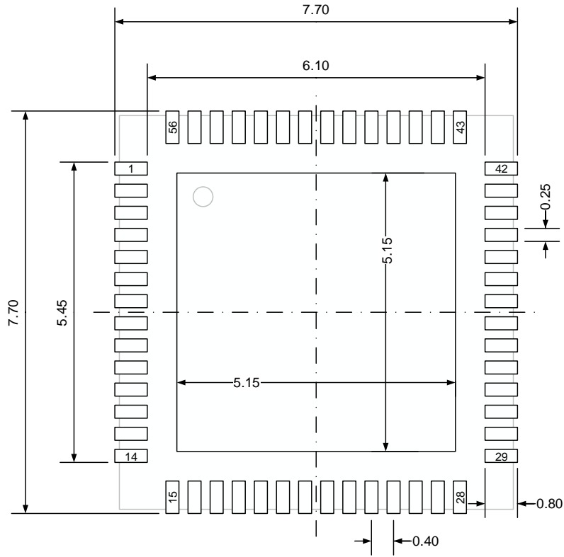
Figure 5-2. QFN56 recommended footprint
