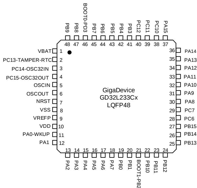
Figure 2-4. GD32L233Cx LQFP48 pinouts
