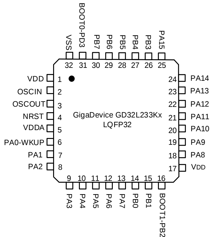
Figure 2-6. GD32L233Kx LQFP32 pinouts
