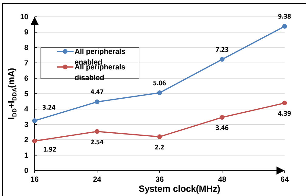
Figure 4-3. Typical supply current consumption in Sleep mode
