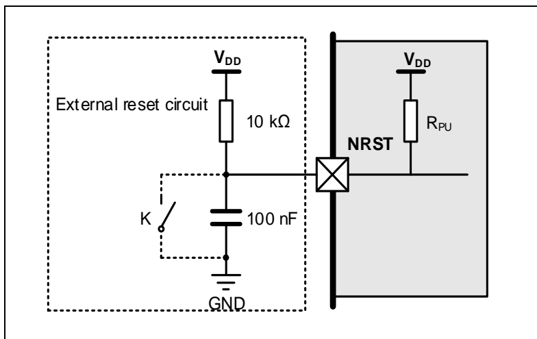
Figure 4-4. Recommended external NRST pin circuit (1)
