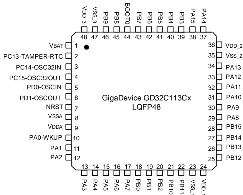
Figure 2-4. GD32C113Cx LQFP48 pinouts
