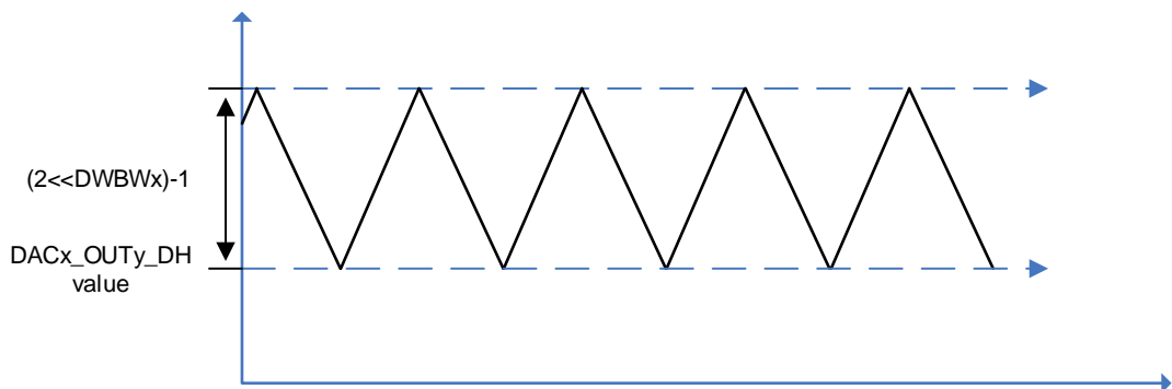
Figure 15-3. DAC triangle noise wave
