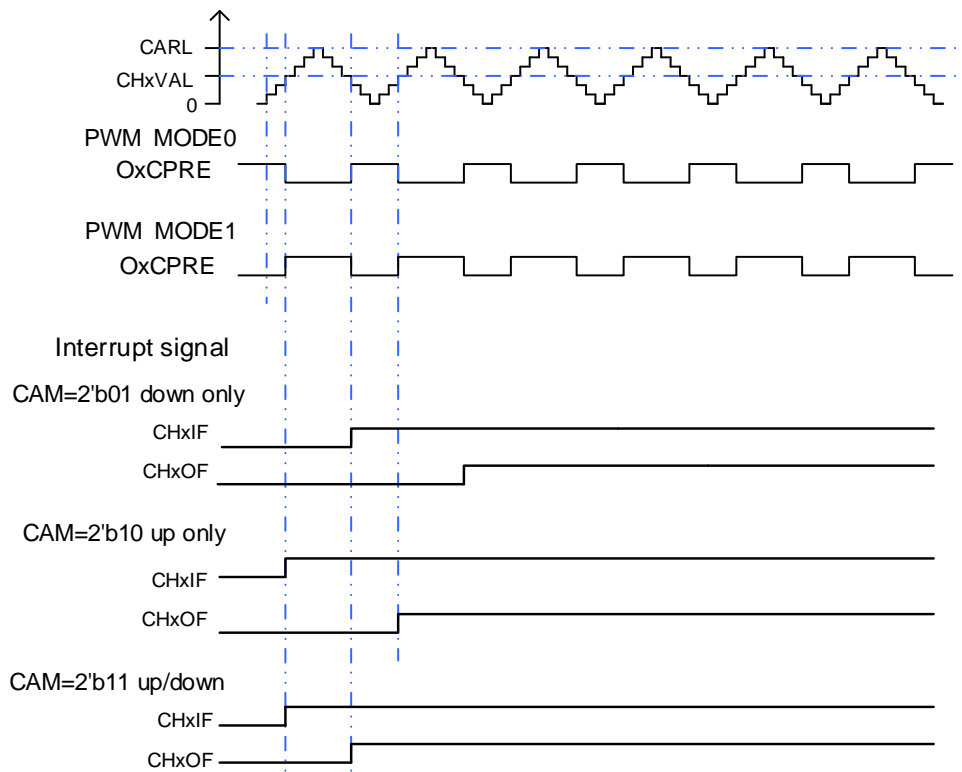
Figure 18-19. CAPWM timechart
