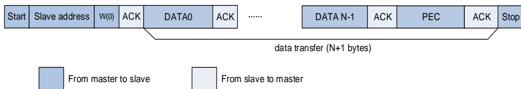
Figure 20-22. SMBus Master Transmitter and Slave Receiver communication flow
