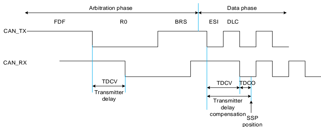
Figure 23-2. Transmitter delay
