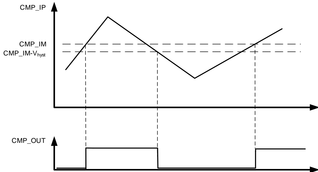
Figure 22-2. CMP hysteresis
