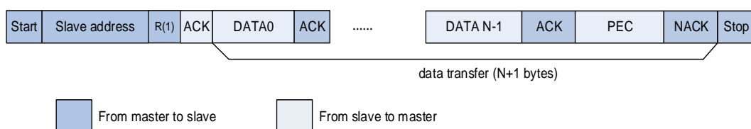
Figure 20-23. SMBus Master Receiver and Slave Transmitter communication flow
