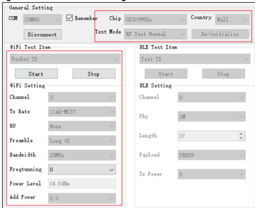
Figure 3-2. Packet TX Tool setting
