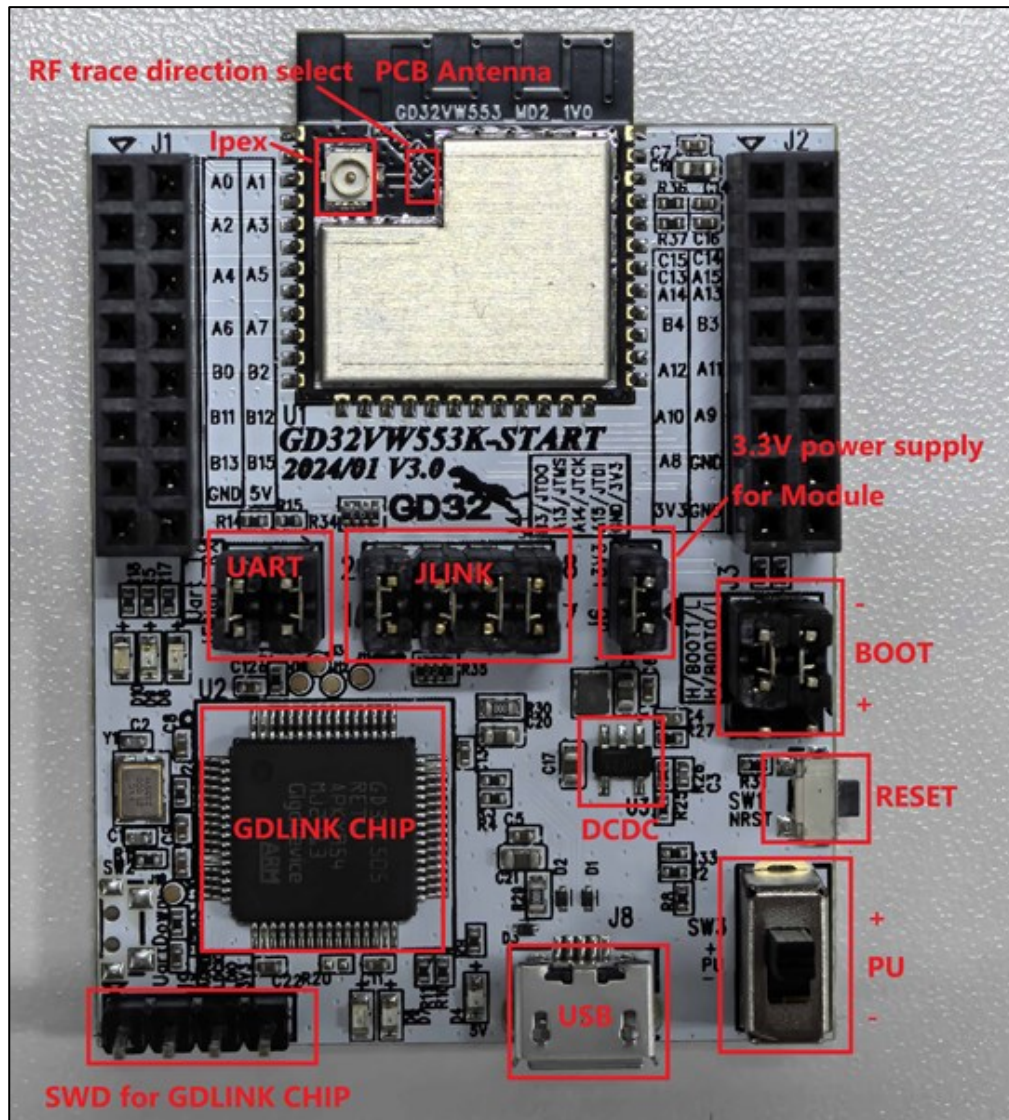
GigaDevice Figure 2-2. Reference connection of GD development board
