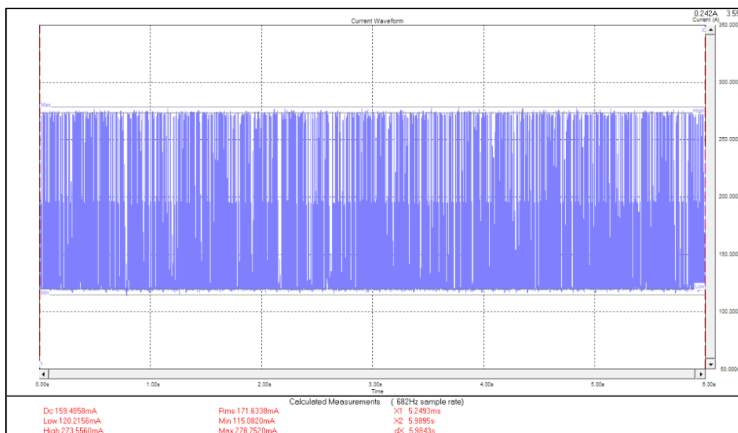
Figure 4-3. "UDP TX" power consumption
