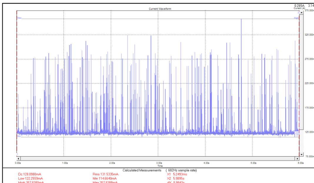
Figure4-4. "UDP RX" power consumption
