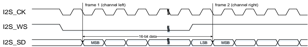
Figure 21-15. I2S Phillips standard timing diagram (DTLEN=00, CHLEN=0, CKPL=1)
