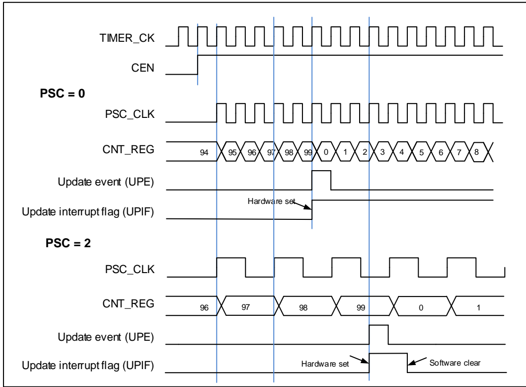
Figure 18-46. Timing chart of up counting mode, PSC=0/2
