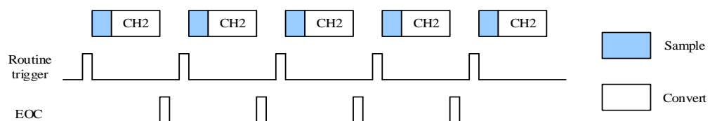
Figure 14-2. Single operation mode
