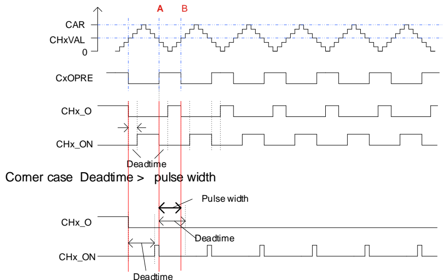
Figure 18-16. Complementary output with dead-time insertion.
