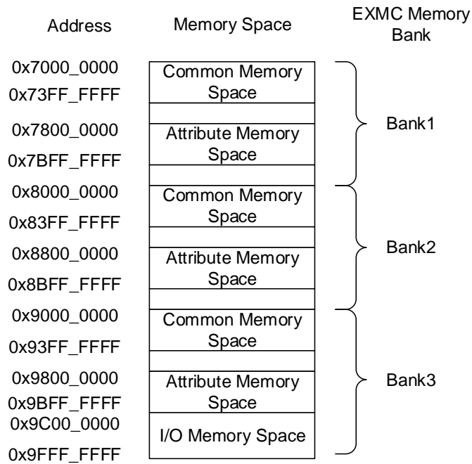
Figure 25-4. NAND/PC card address mapping
