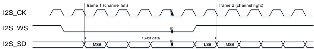
Figure 21-14. I2S Phillips standard timing diagram (DTLEN=00, CHLEN=0, CKPL=0)
