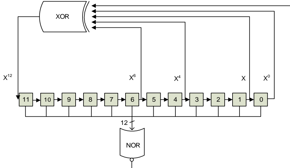
Figure 15-2. DAC LFSR algorithm
