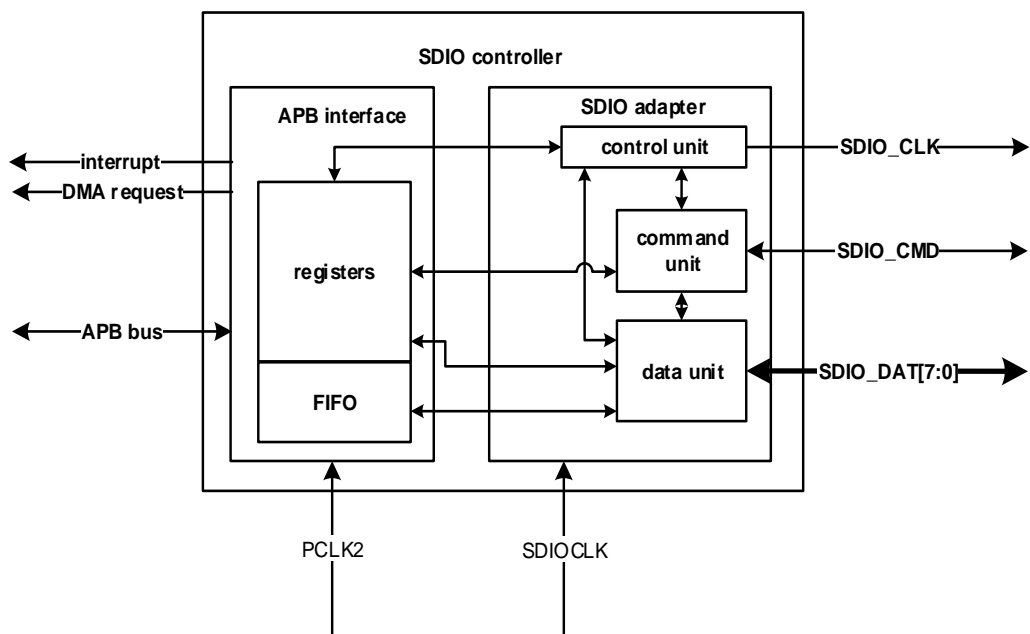
Figure 24-6. SDIO block diagram
