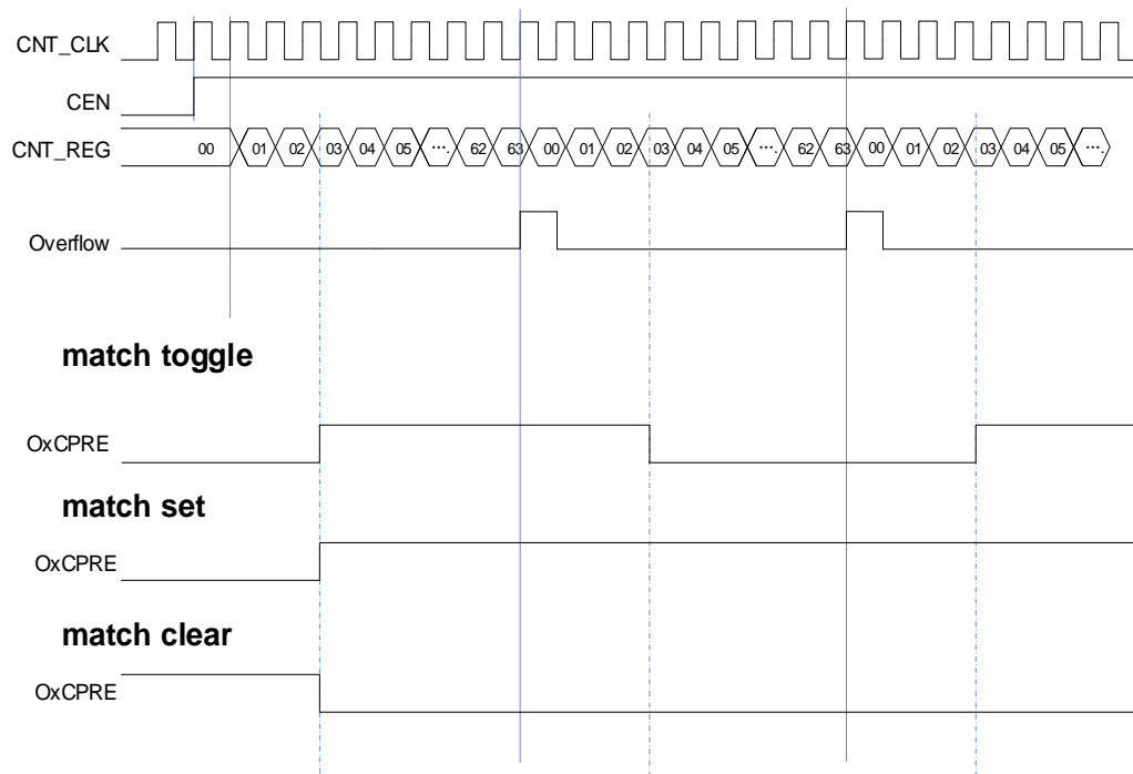
Figure 18-49. Output-compare under three modes
