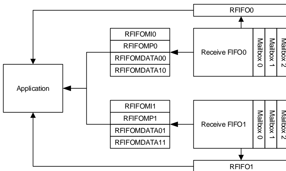
Figure 26-4. Reception register
