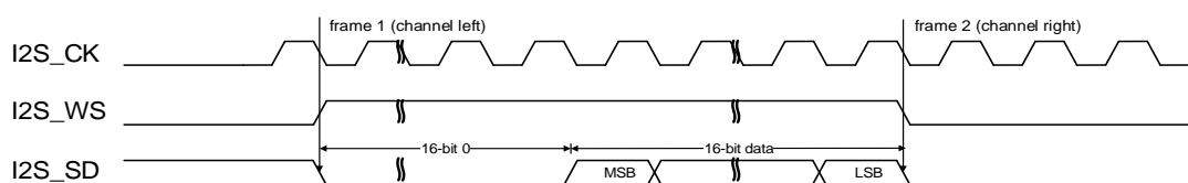
Figure 21-32. LSB justified standard timing diagram (DTLEN=00, CHLEN=1, CKPL=0)
