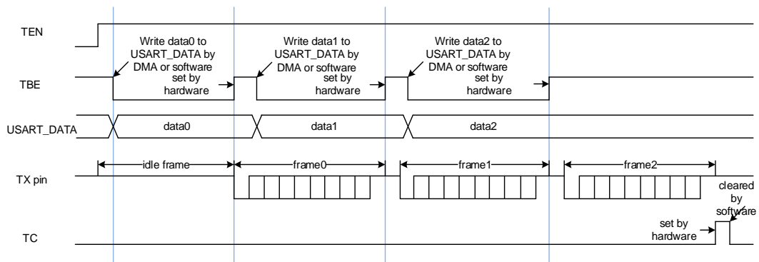
Figure 19-3. USART transmit procedure
