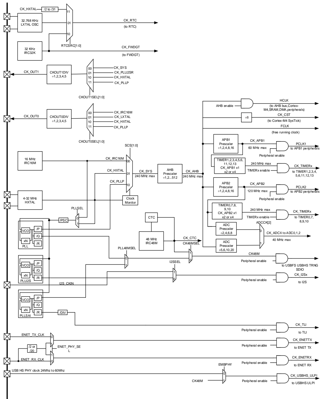
Figure 4-2. Clock tree
