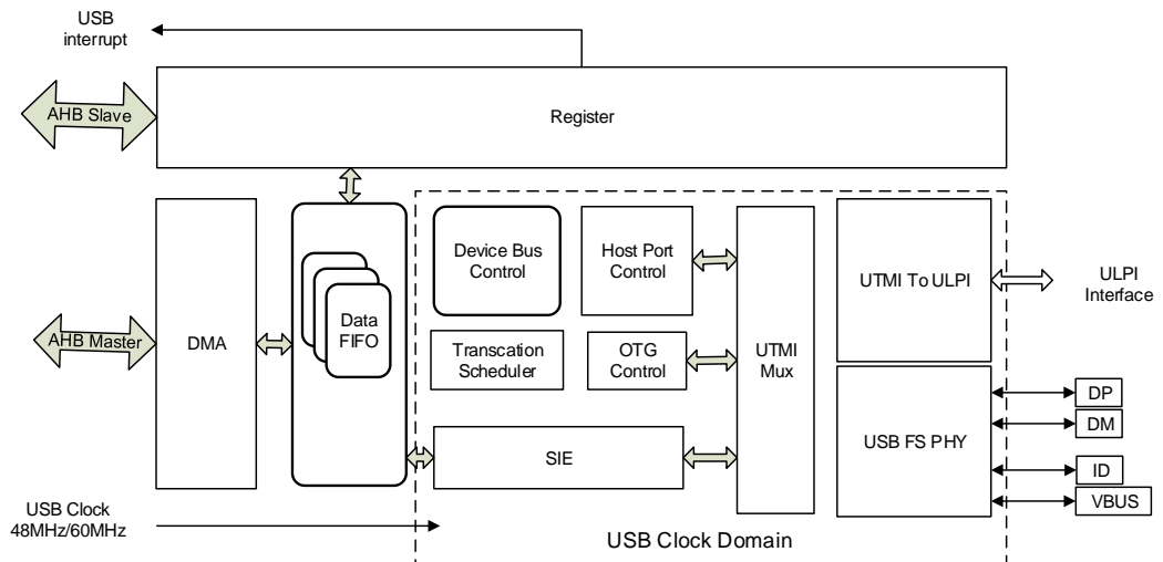
Figure 29-1. USBHS block diagram
