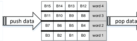
Figure 10-5. Data packing/unpacking when PWIDTH = '01'
