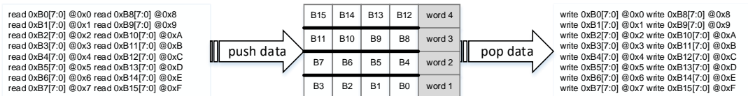
Figure 10-4. Data packing/unpacking when PWIDTH = '00'
