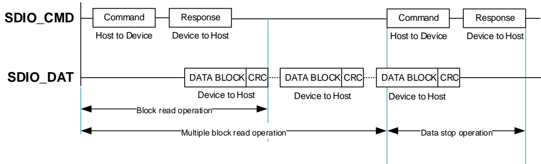
Figure 24-2. SDIO multiple blocks read operation
