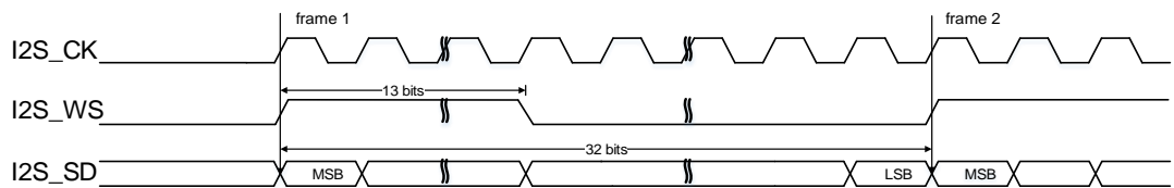
Figure 21-44. PCM standard long frame synchronization mode timing diagram (DTLEN=10, CHLEN=1, CKPL=0)
