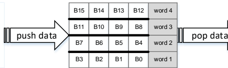
Figure 10-6. Data packing/unpacking when PWIDTH = '10'
