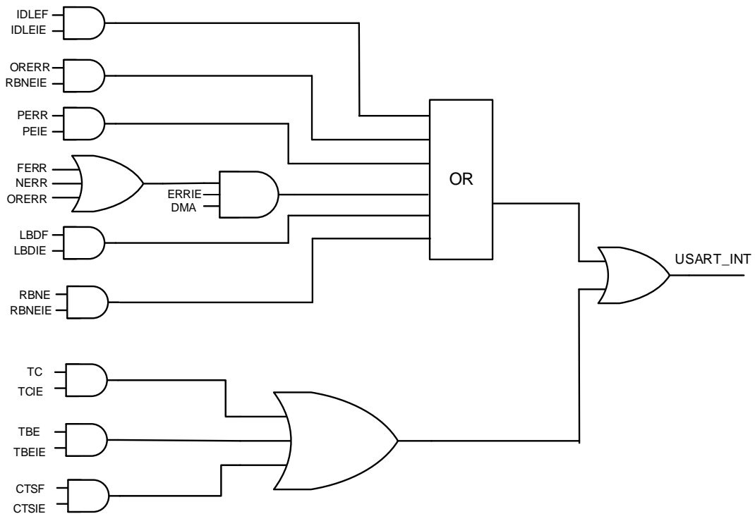
Figure 19-16. USART interrupt mapping diagram
