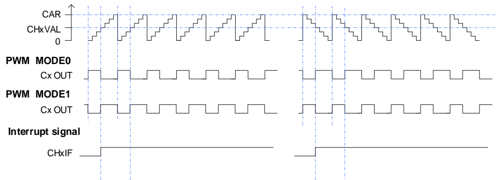
Figure 18-51. CAPWM timechart
