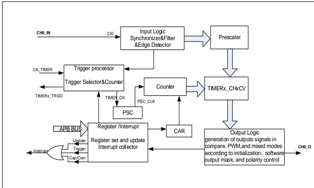
Figure 18-56. General level2 timer block diagram
