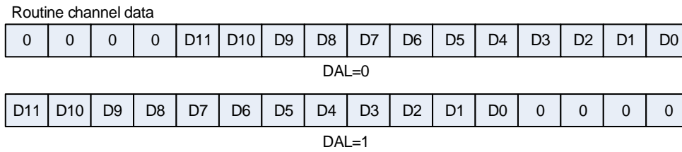
Figure 14-8. Data storage mode of 10-bit resolution
