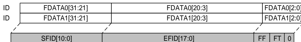
Figure 26-9. 32-bit list mode filter
