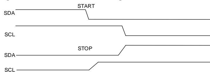
Figure 20-3. START and STOP signal
