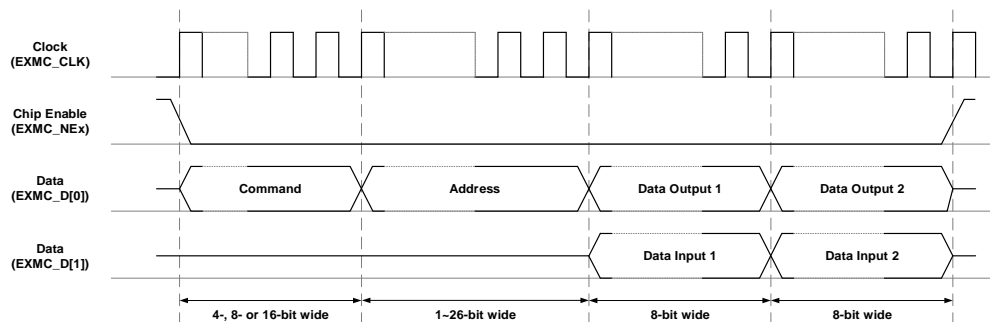
Figure 25-24. SPI-PSRAM access
