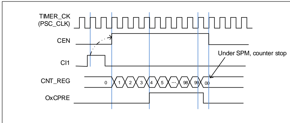
Figure 18-55. Single pulse mode TIMERx\_CHxCV = 4 TIMERx\_CAR=99
