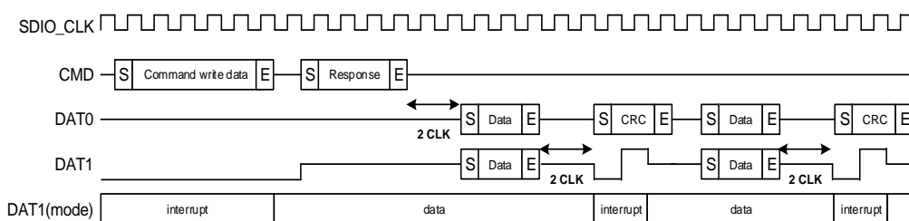
Figure 24-18. Multiple block 4-Bit write interrupt cycle timing
