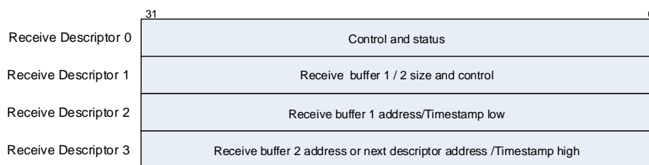
Figure 27-9. Receive descriptor in normal mode
