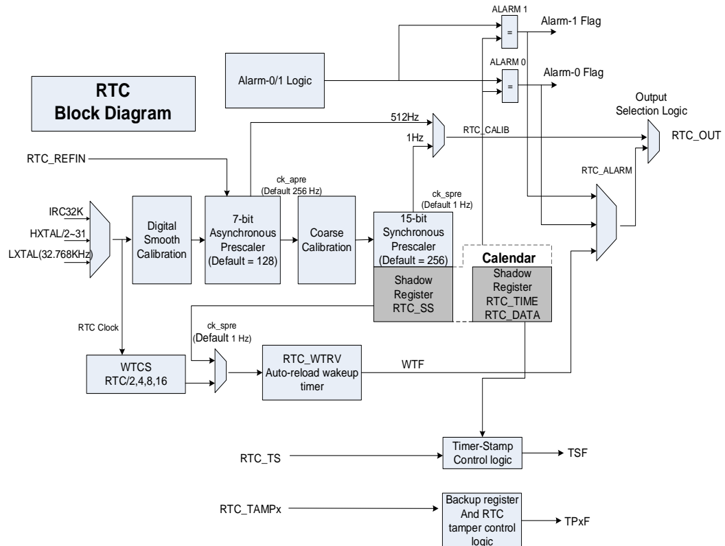
Figure 17-1. Block diagram of RTC
