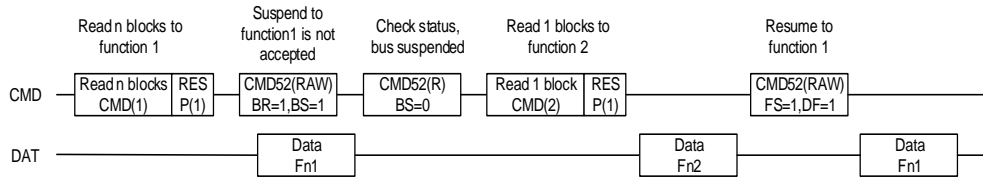
Figure 24-14. Function2 read cycle inserted during function1 multiple read cycle
