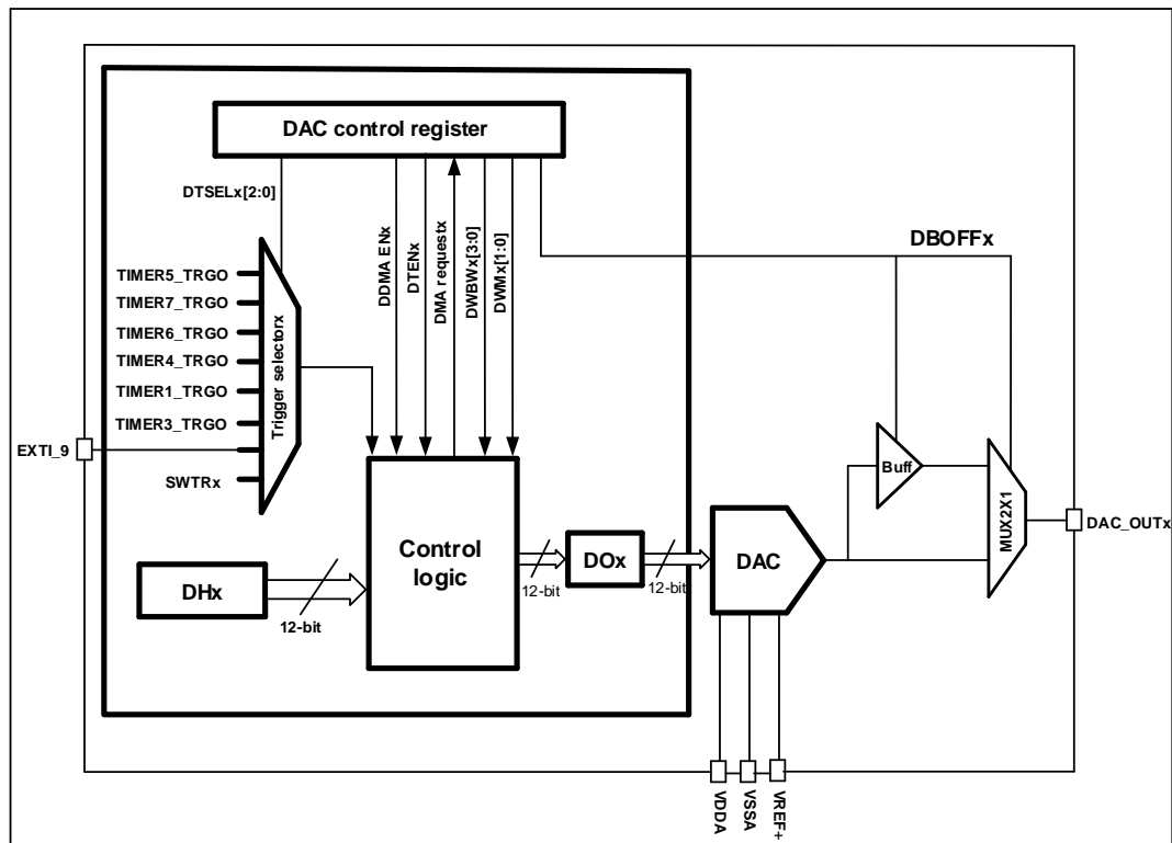
Figure 15-1. DAC block diagram
