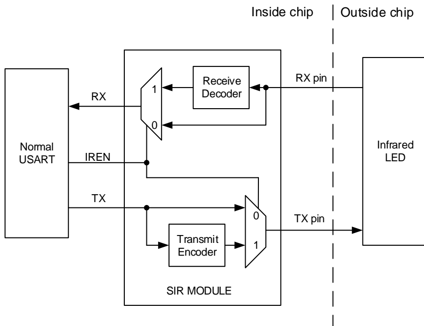
Figure 19-13. IrDA SIR ENDEC module
