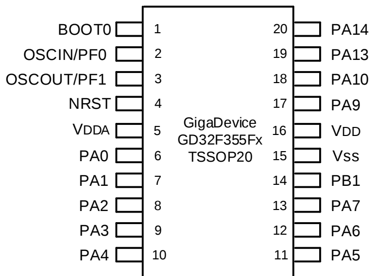
Figure 2-7. GD32F355Fx TSSOP20 pinouts
