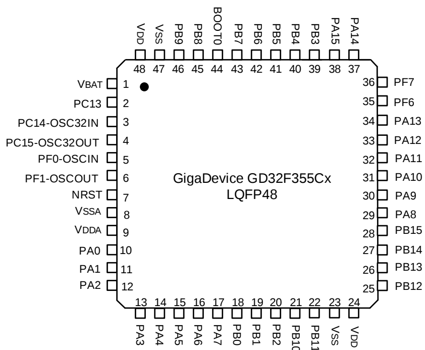
Figure 2-3. GD32F355Cx LQFP48 pinouts
