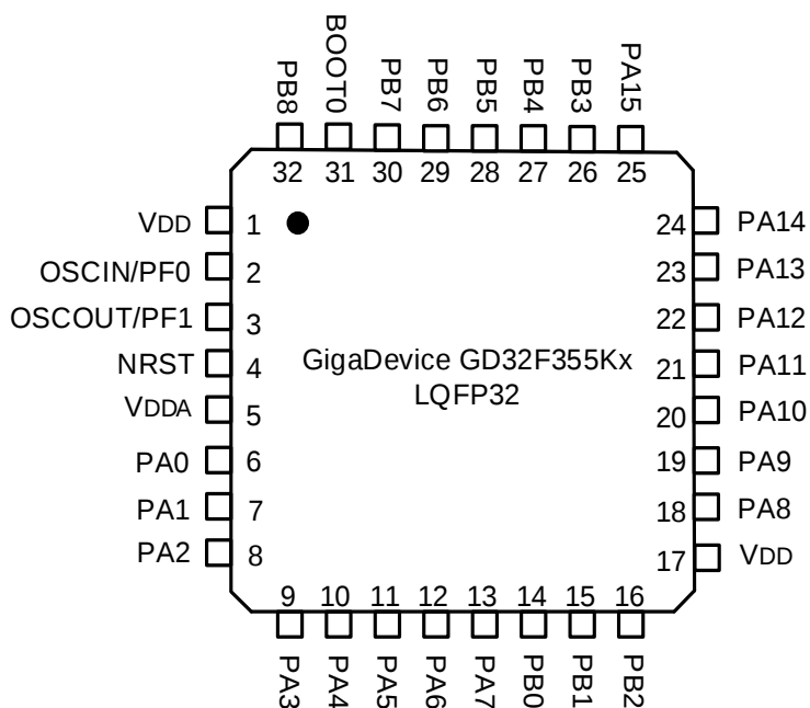
Figure 2-5. GD32F355Kx QFN32 pinouts
