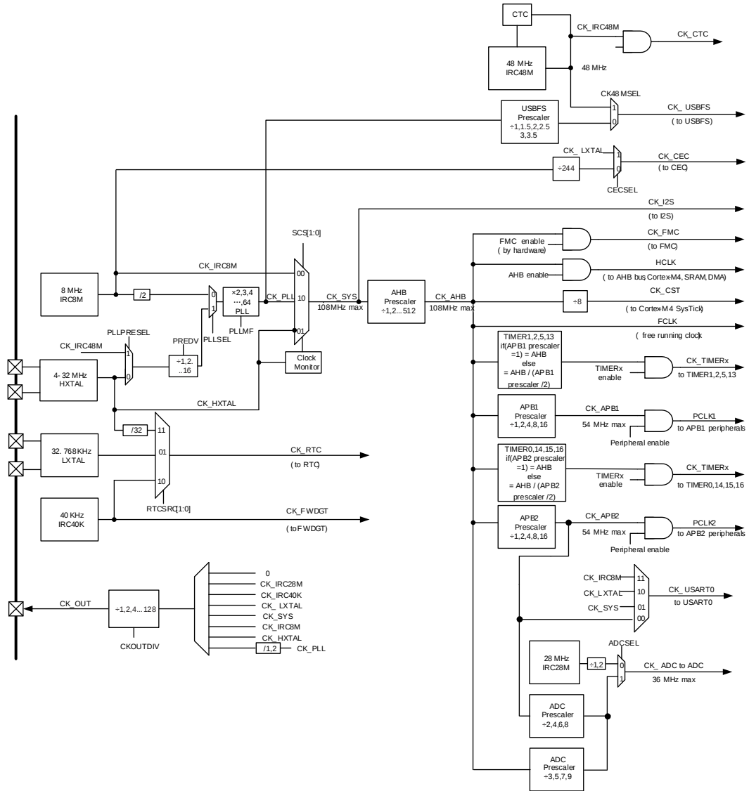
Figure 2-8. GD32F355xx clock tree
